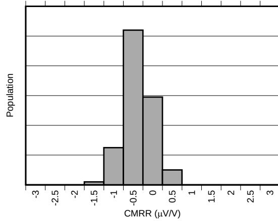
Figure 7. Common-Mode Rejection Ratio Distribution (INA301A3-Q1)
