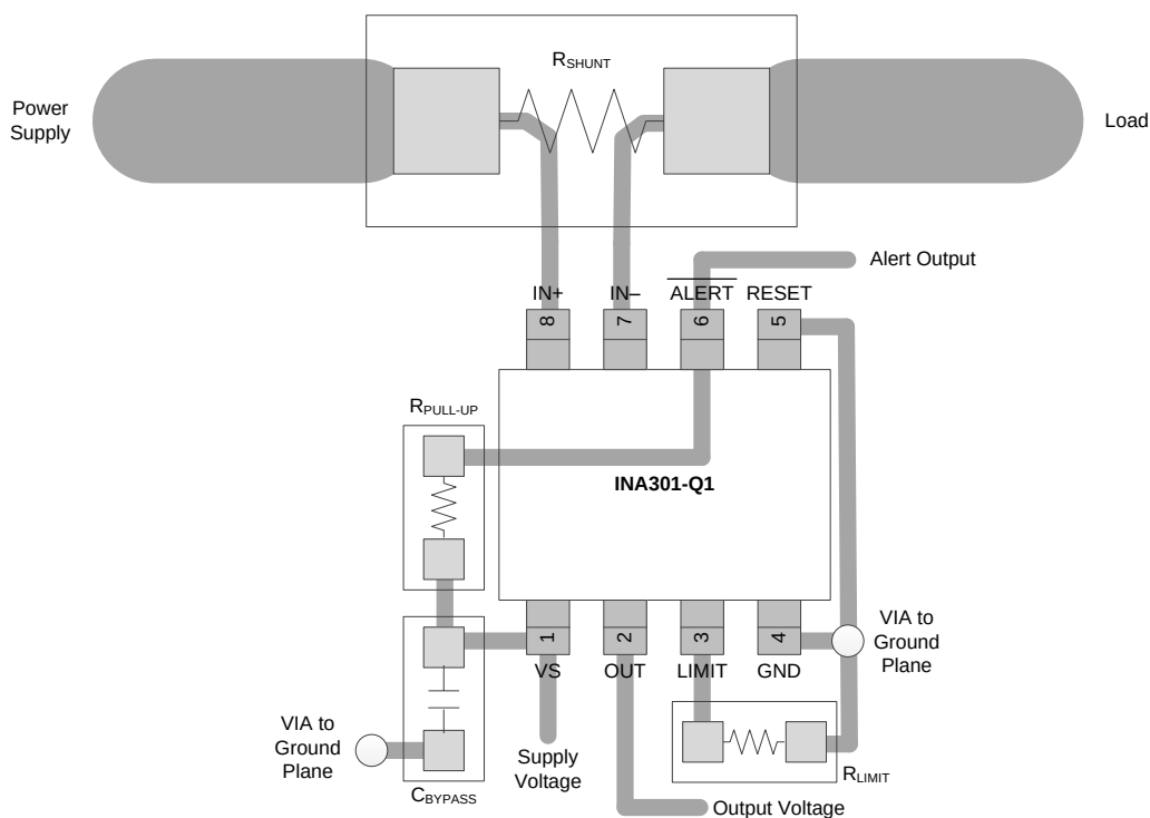
Figure 44. Recommended Layout
