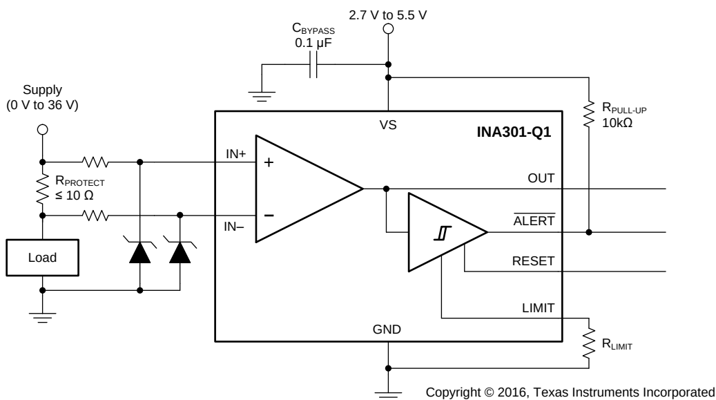
Figure 41. Transient Protection
