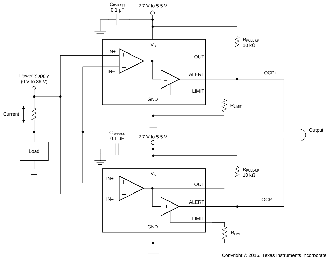
Figure 42. Bidirectional Application
