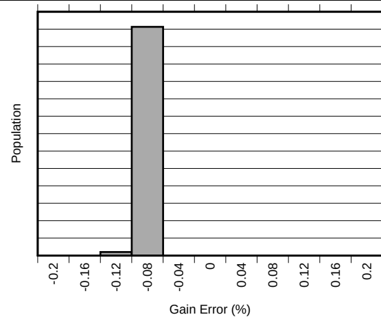
Figure 10. Gain Error Distribution (INA301A1-Q1)
