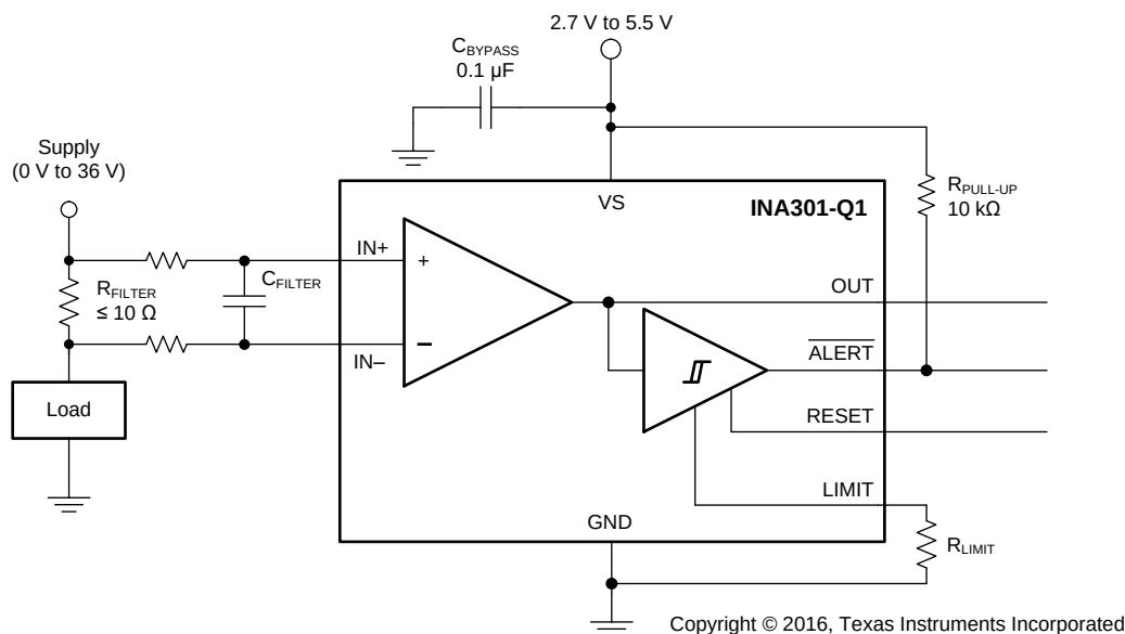
Figure 39. Input Filter
