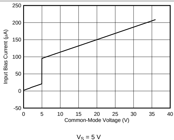
Figure 17. Input Bias Current vs Common-Mode Voltage
