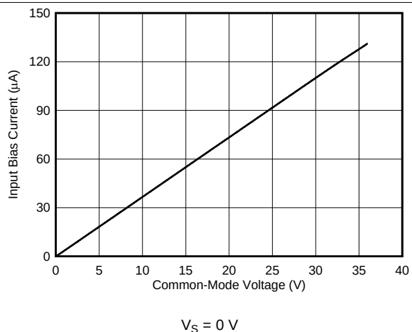
Figure 18. Input Bias Current vs Common-Mode Voltage
