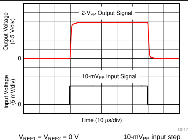
Figure 20. Step Response
