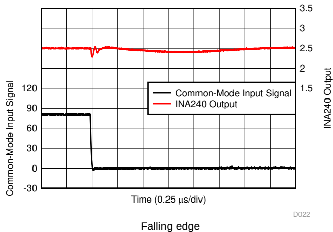
Figure 22. Common-Mode Voltage Transient Response
