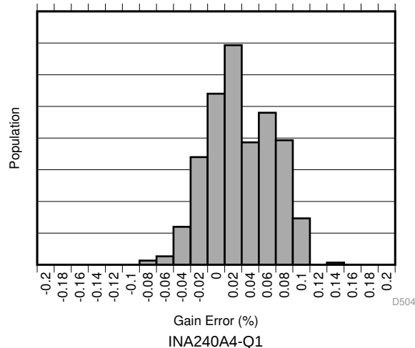
Figure 8. Gain Error Production Distribution
