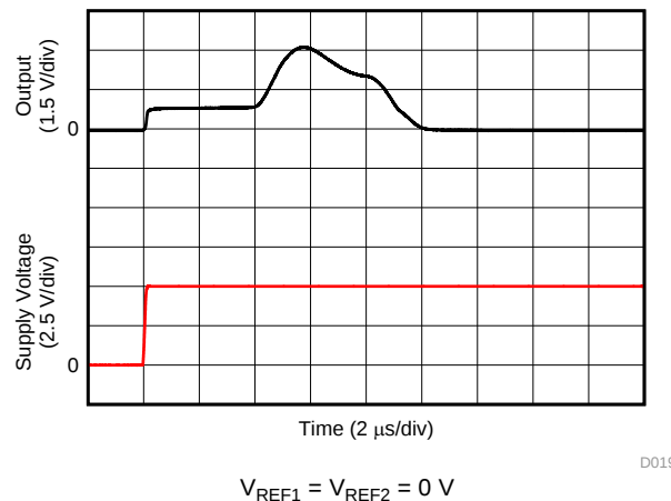
Figure 23. Start-Up Response
