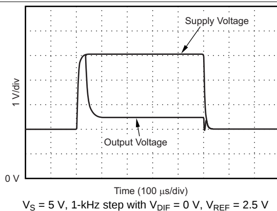
Figure 19. Brownout Recovery
