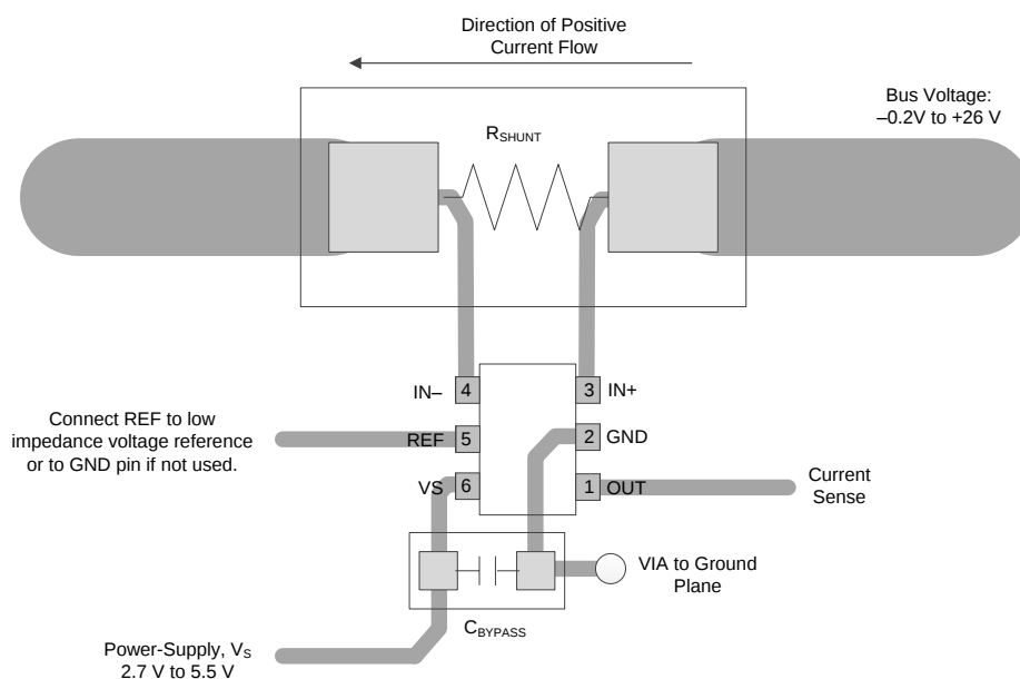
Figure 44. Recommended Layout
