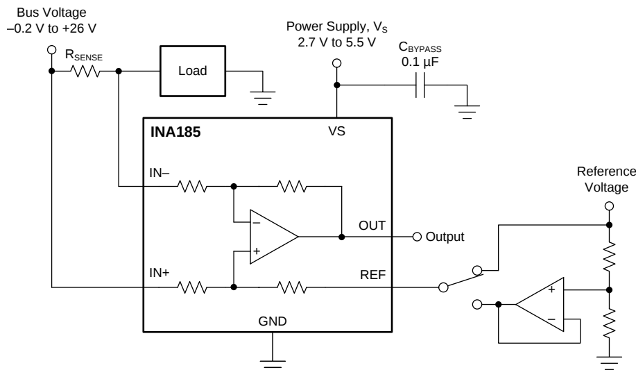
Figure 36. Bidirectional Application
