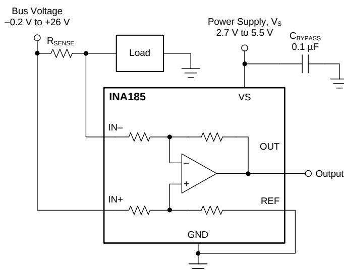
Figure 35. Unidirectional Application
