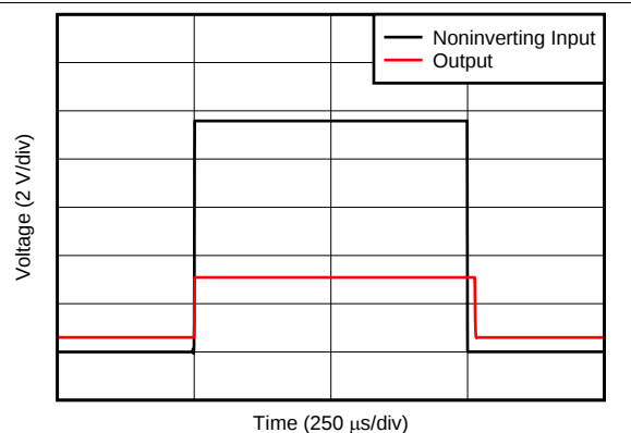
Figure 28. Common-Mode Voltage Transient Response
