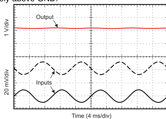
Figure 52. Current Differencing Application Output Response (A2 Devices)
