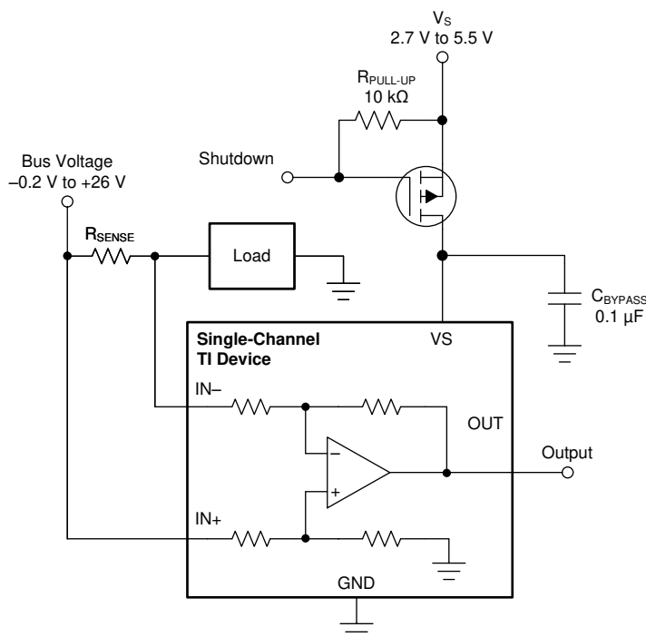
Figure 44. Basic Circuit to Shut Down the INAx180
