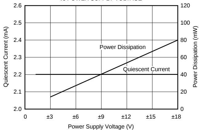
QUIESCENT CURRENT AND POWER DISSIPATION vs POWER SUPPLY VOLTAGE
