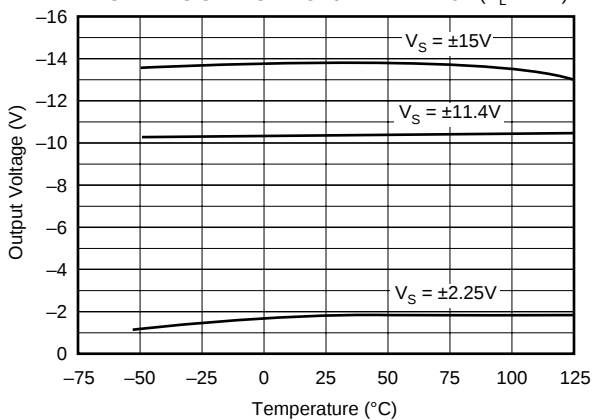
NEGATIVE SIGNAL SWING vs TEMPERATURE ( R_L = 2k\Omega )
