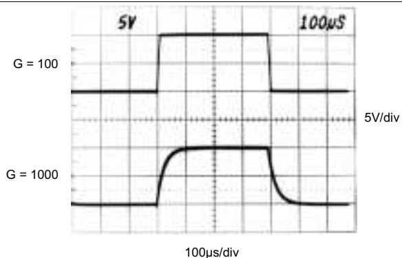
Figure 22. Small-Signal Response
