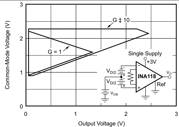
Figure 4. Input Common-Mode Range vs Output Voltage
