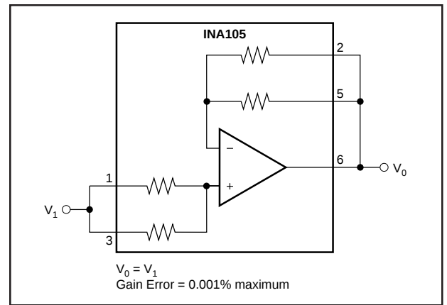
FIGURE 9. Precision Unity-Gain Buffer.
