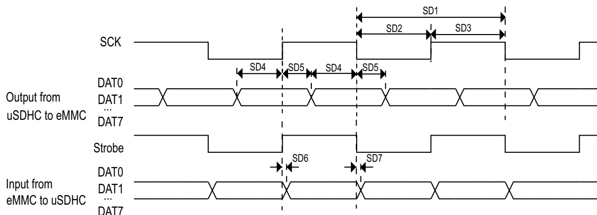
Figure 43. HS400 timing
