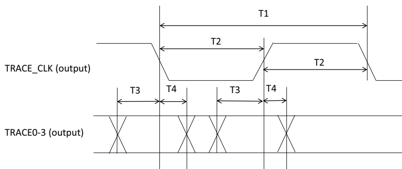
Figure 14. Trace timing
