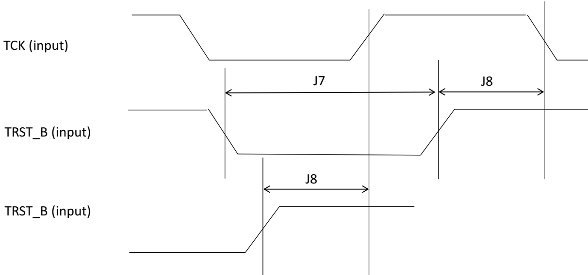
Figure 12. JTAG_TRST_B timing
