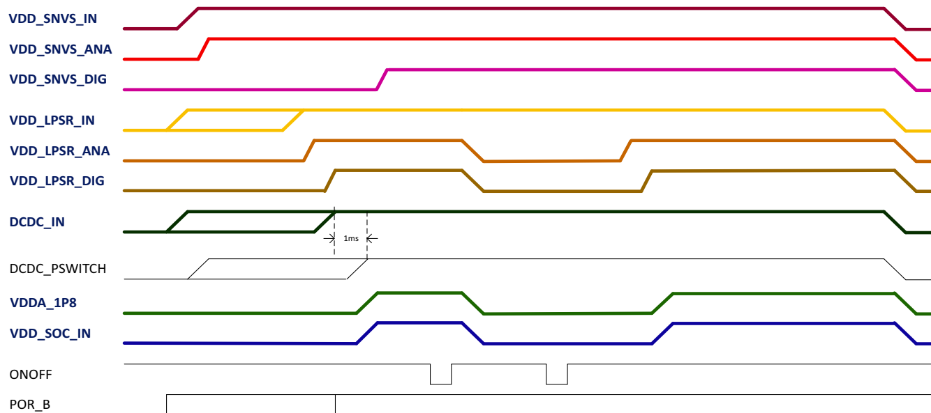
Figure 4. Power sequence
