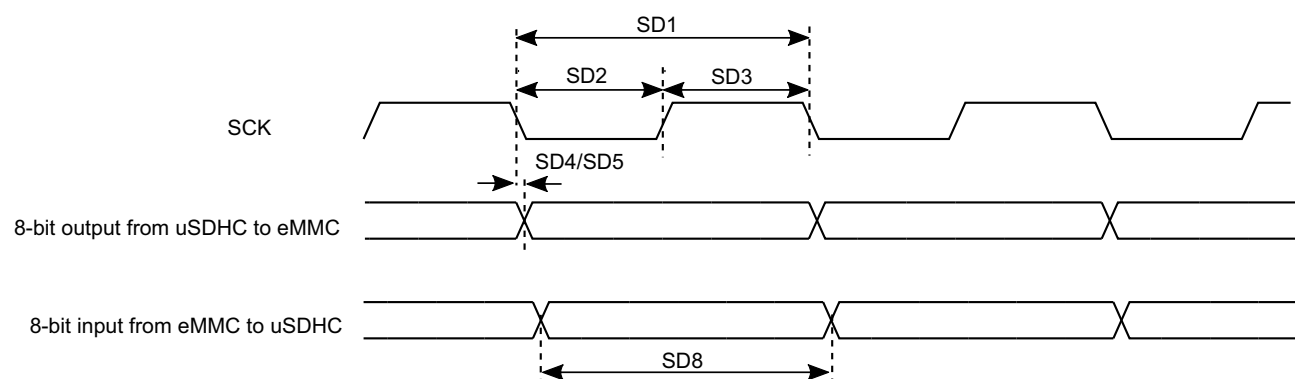
Figure 15. HS200 timing
