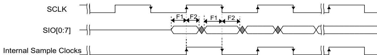
Figure 37. FlexSPI input timing in DDR mode where FlexSPIn_MCR0[RXCLKSRC] = 0x0, 0x1, 0x2
