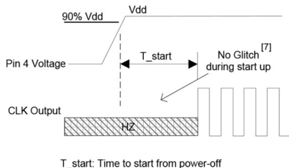
Figure 9: Startup Timing (OE/ST Mode)
