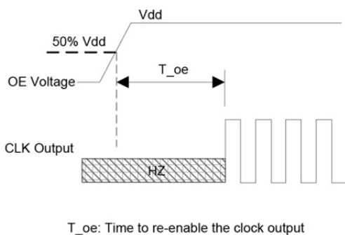
Figure 11: OE Enable Timing (OE Mode Only)
