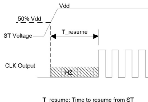
Figure 10: Standby Resume Timing (ST Mode Only)
