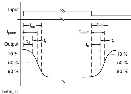
Fig. 11 - Saturated Switching Time Test Waveform
