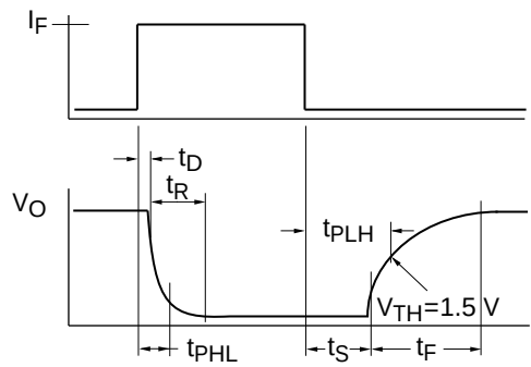
Figure 9. Switching timing
