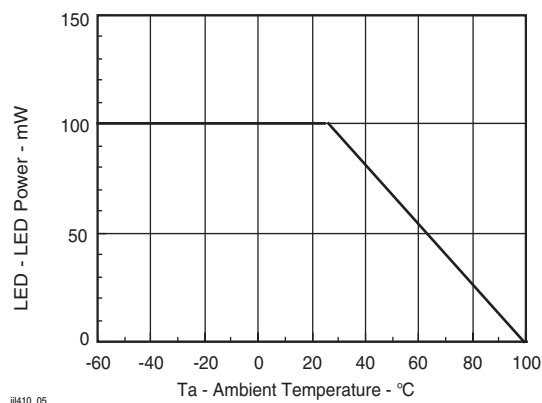
Figure 5. Maximum LED Power Dissipation
