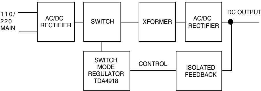
Figure 17. Switching Mode Power Supply
