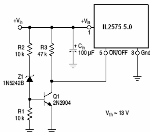
Figure 21. Undervoltage Lockout Circuit for Buck Converter
