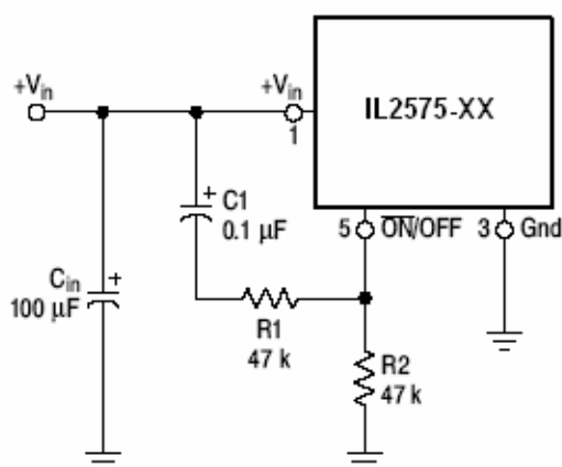
Figure 20. Delayed Startup Circuitry
