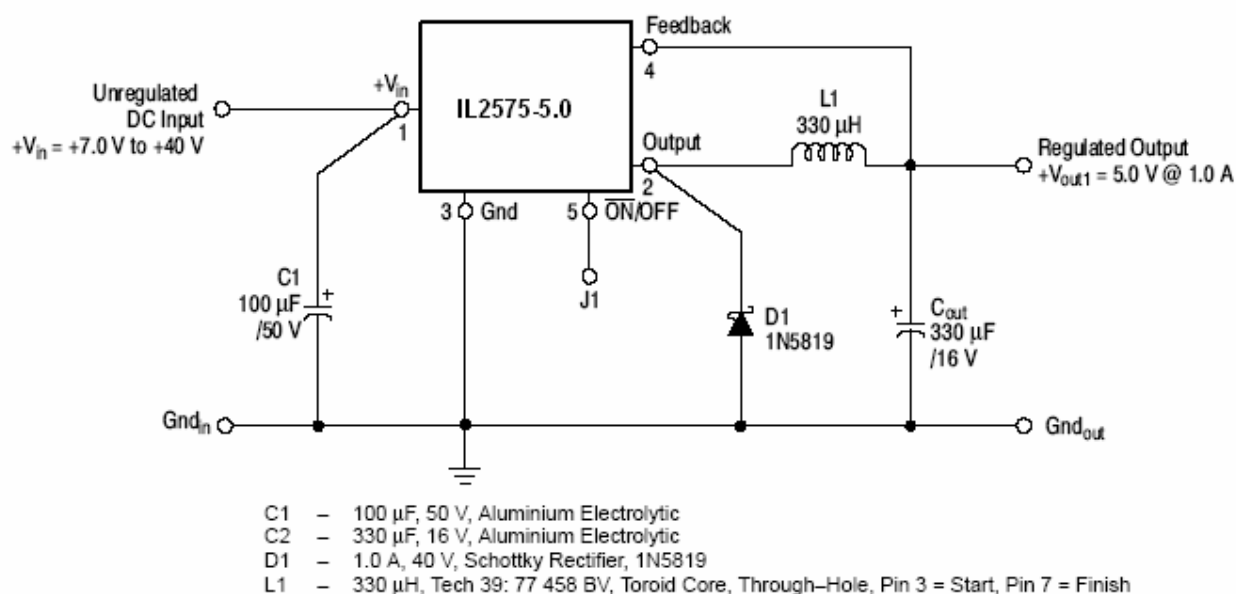
Figure 25. Schematic Diagram of the IL2575-5.0 Step-Down Converter
