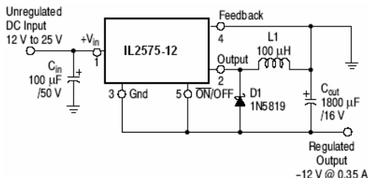
Figure 15. Inverting Buck-Boost Regulator Using the IL2575-12 Develops -12 V @ 0.35 A
