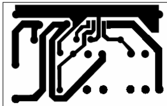
Figure 30. PC Board Copper Side
