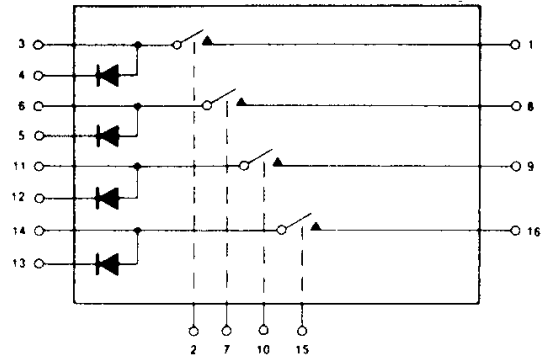
IH5011, IH5012 (16 LEAD CERDIP, 16 LEAD PDIP)
