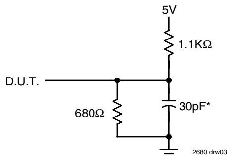
Figure 1. Output Load
