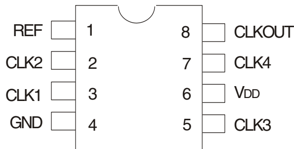
SOIC TOP VIEW
