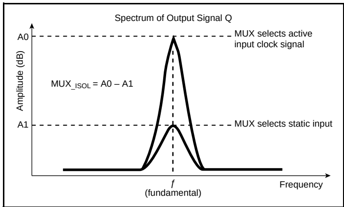
MUX Isolation
