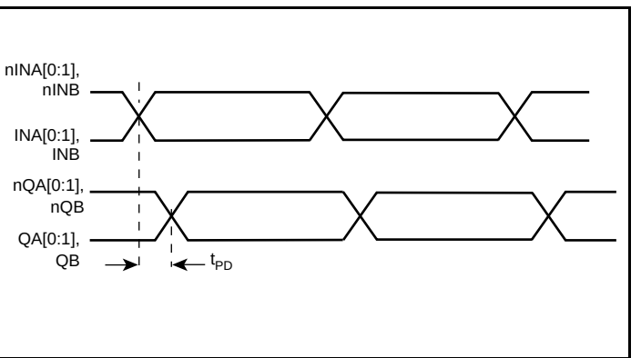
Propagation Delay
