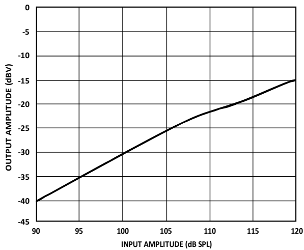
Figure 7. Linearity
