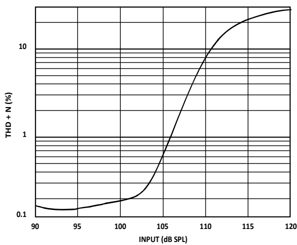
Figure 6. THD + N vs. Input Level
