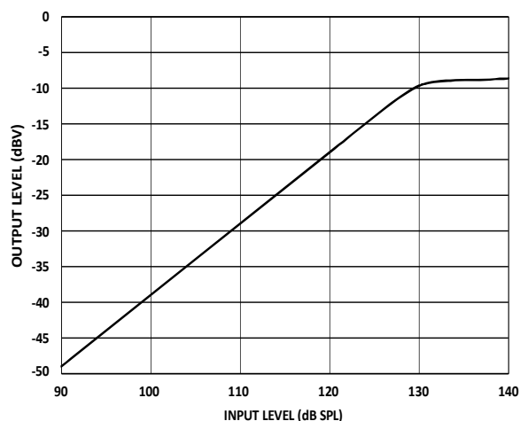
Figure 6. Linearity
