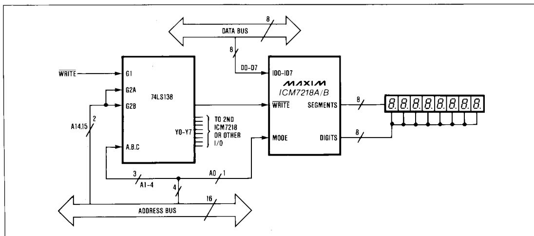
Figure 8. ICM7218A/B μP Bus Interface
