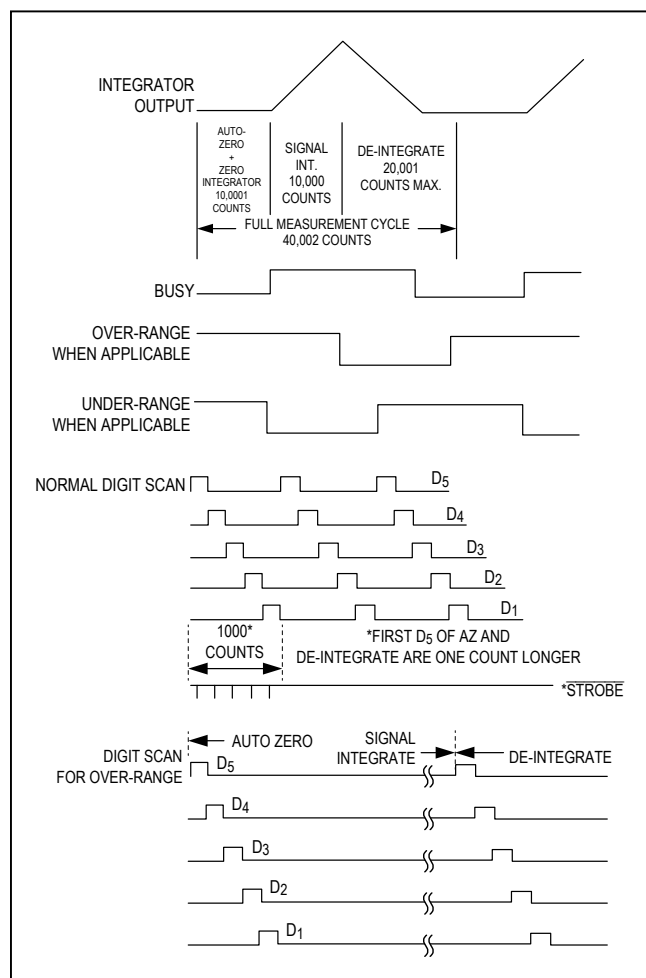
Figure 4. Timing Diagram
