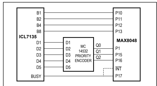
Figure 13. \mu P Interface
