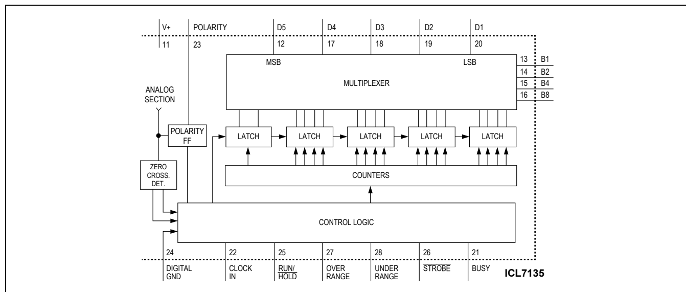
Figure 3. ICL7135 Digital Section
