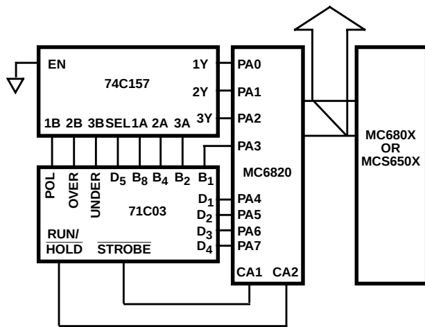
FIGURE 18. ICL71C03 TO MC6800, MCS650X INTERFACE
