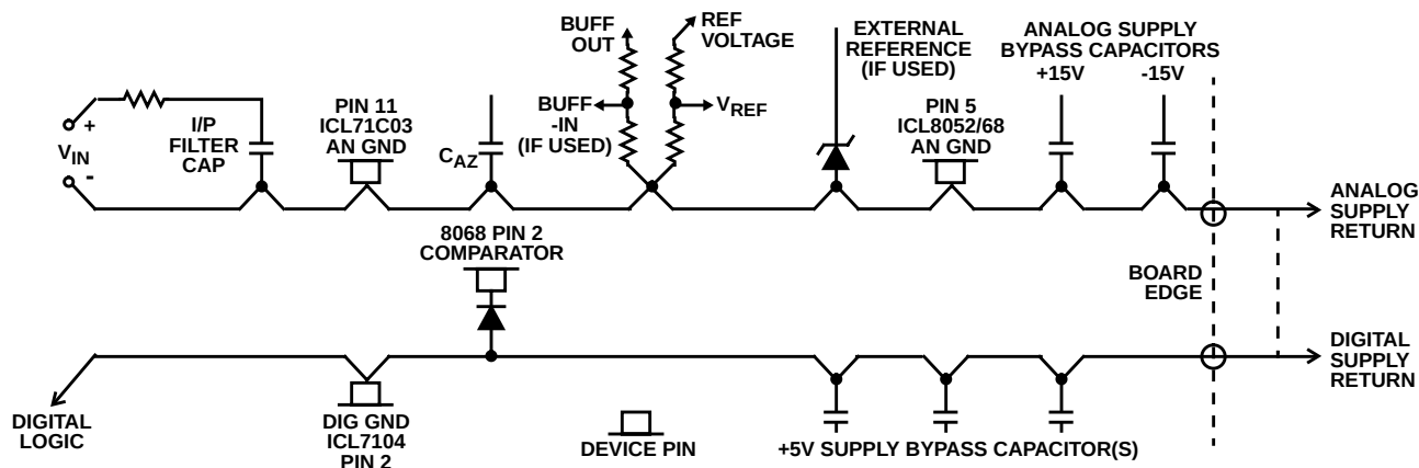
FIGURE 9. GROUNDING SEQUENCE
