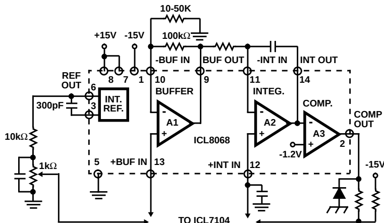
FIGURE 6. ADDING BUFFER GAIN TO ICL8068
