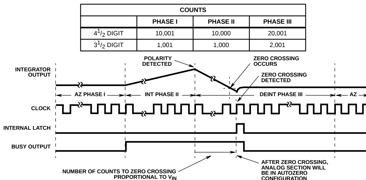
FIGURE 3. CONVERSION TIMING
