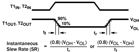
FIGURE 7. SLEW RATE DEFINITION
