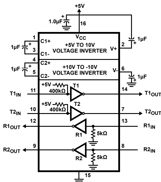
FIGURE 1. FUNCTIONAL DIAGRAM
