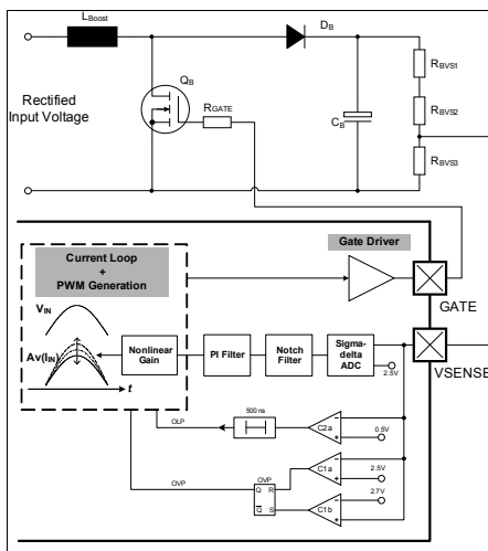
Figure 6 Voltage Loop
