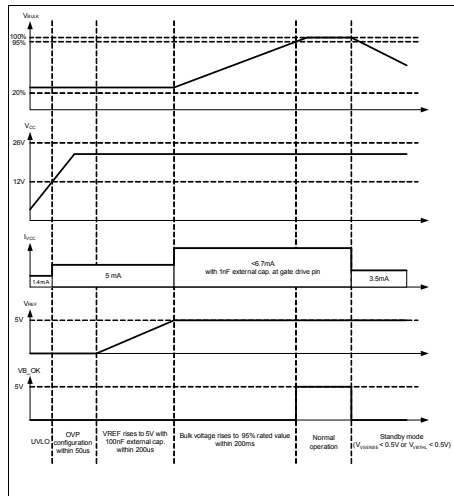
Figure 3 State of Operation respect to VCC
