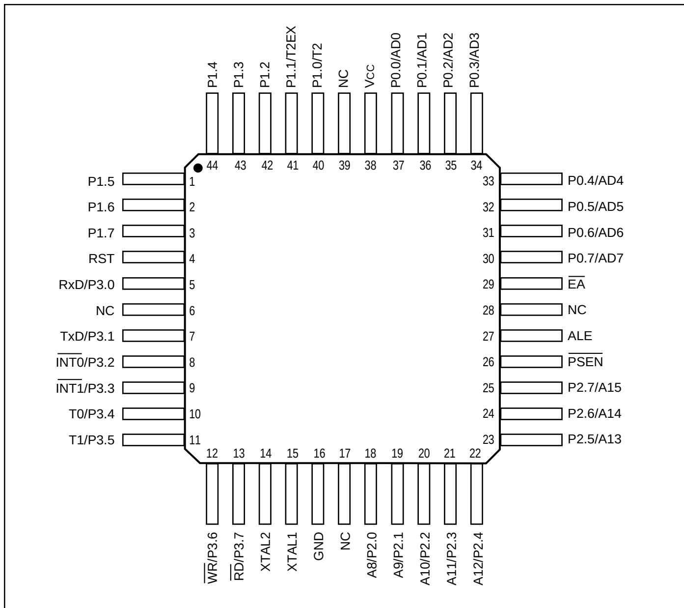
Figure 3. IC80C52/32 Pin Configuration: 44-pin PQFP
