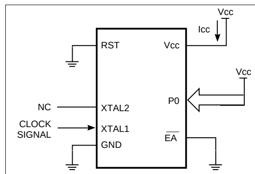
Figure 29. Idle Mode
