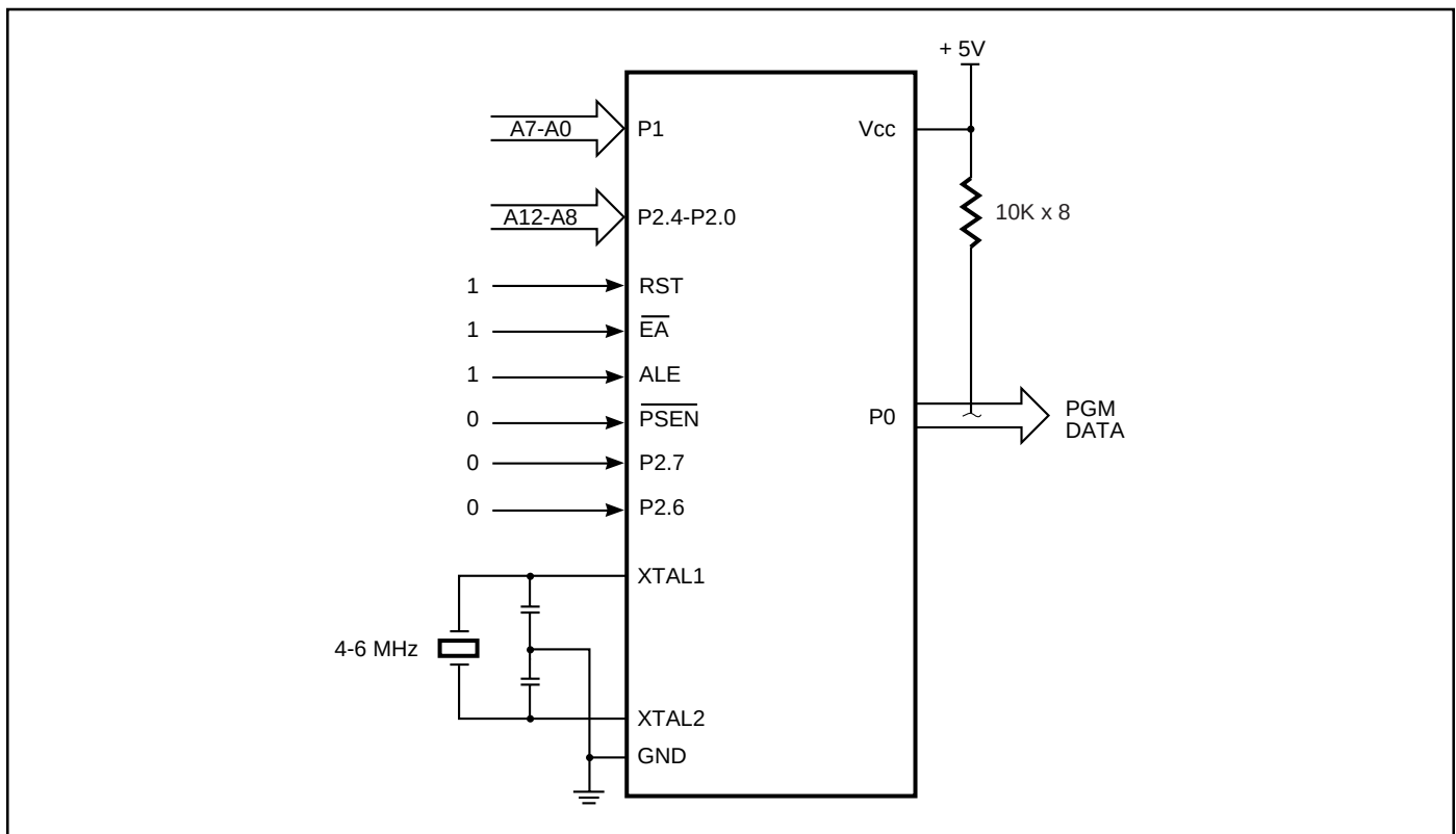
Figure 27. ROM Verification
