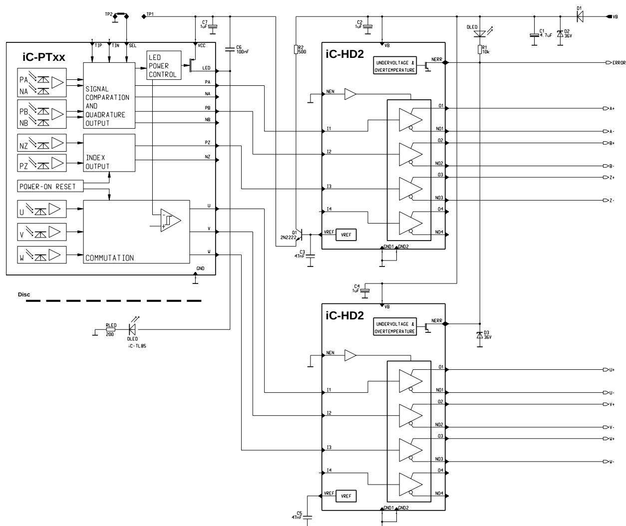
Figure 3: Circuit example of an incremental/commutation encoder with RS422 line drivers for 5V applications.
