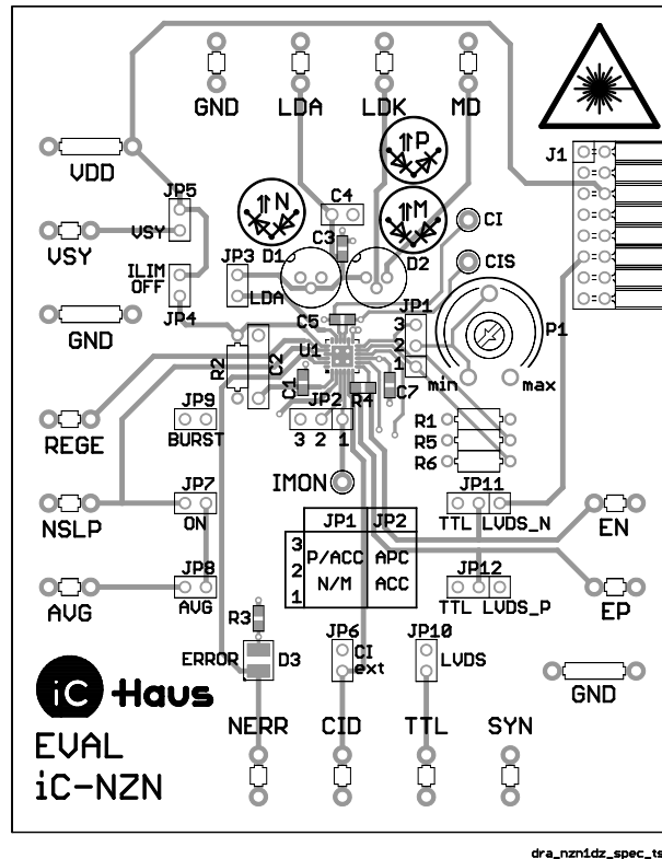
Figure 11: Evaluation board (component side)
