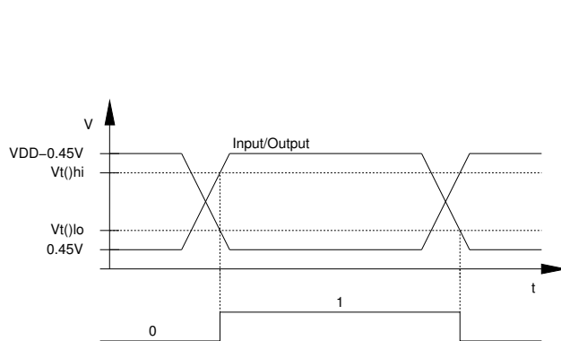
Figure 1: Reference levels
