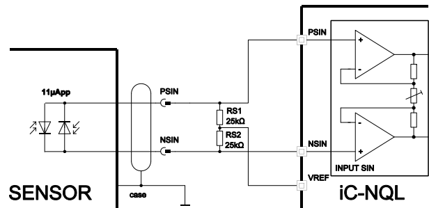
Figure 17: Input circuit for current signals of 11μA. This circuit does not permit offset calibration.
