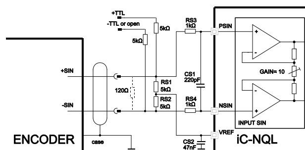
Figure 21: Combined input circuit for 11μA, 1Vpp (with 120Ω termination) or TTL encoder signals. RS3/4 and CS1 serve as protection against ESD and transients.
