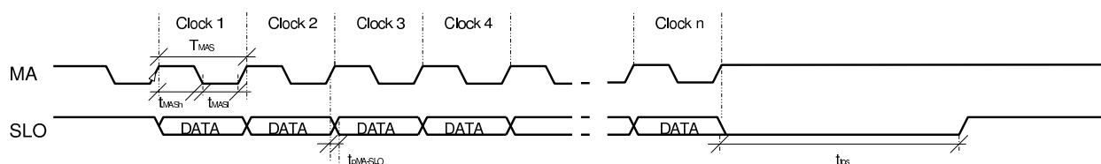
Figure 2: Timing diagram of SSI output.
