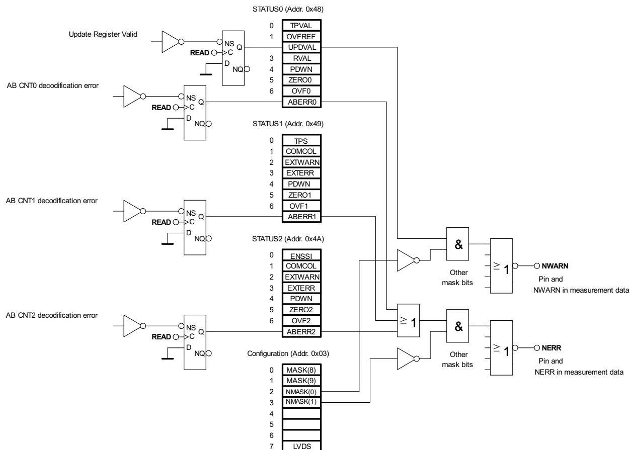
Figure 9: NMASK gating
