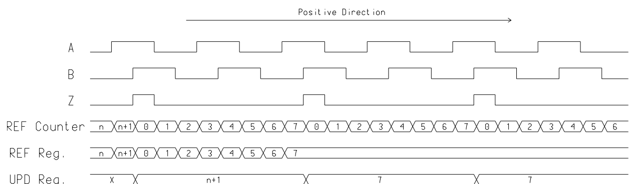
Figure 4: Zero-Codification: REF and UPD registers after activation of Zero Codification function
