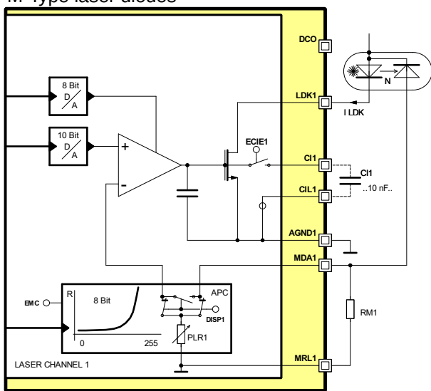
Figure 2: iC-HT with N-type laser diode
