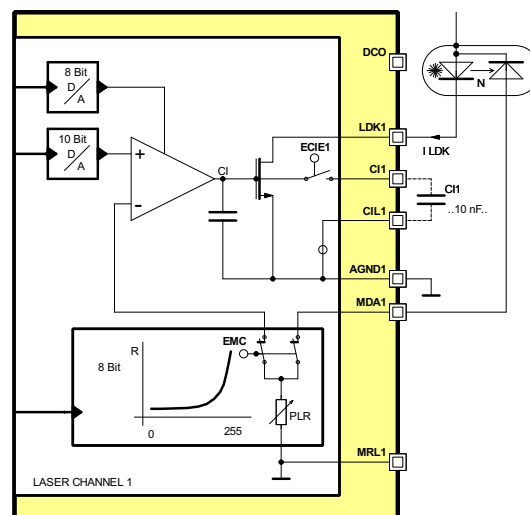
Figure 7: APC mode simplified
