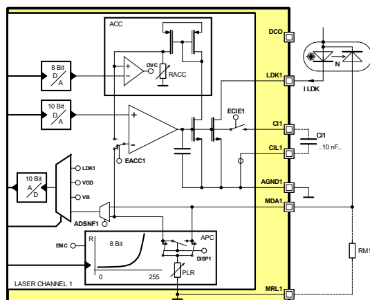
Figure 6: Channel 1 schematic
