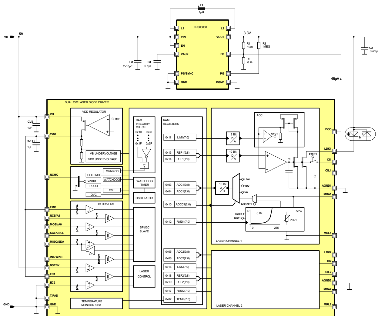
Figure 20: System efficiency enhancement
