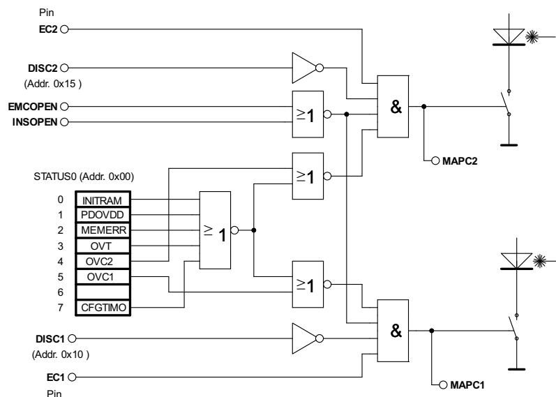
Figure 10: Laser control logic in MCU mode
