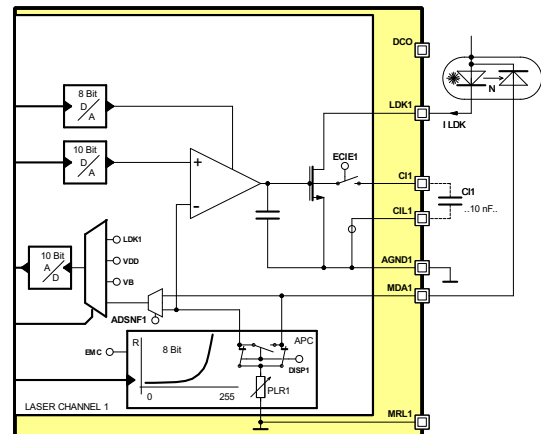
Figure 15: PLR in APC
