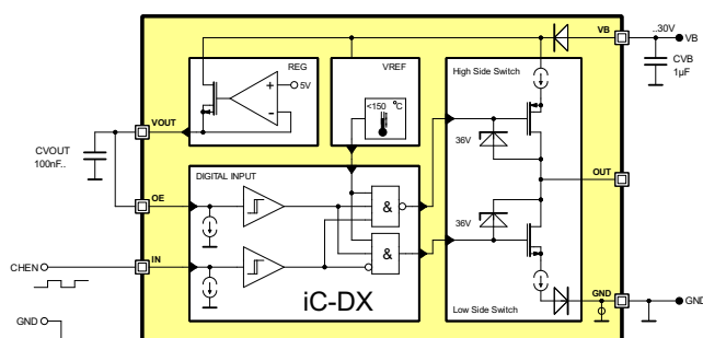
Figure 6: Configuration as Push-Pull
