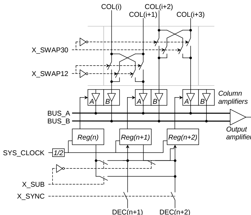
Figure 6. Column Structure
