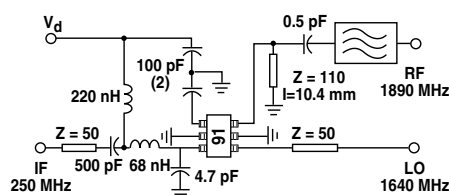
Figure 18. Test Circuit.
