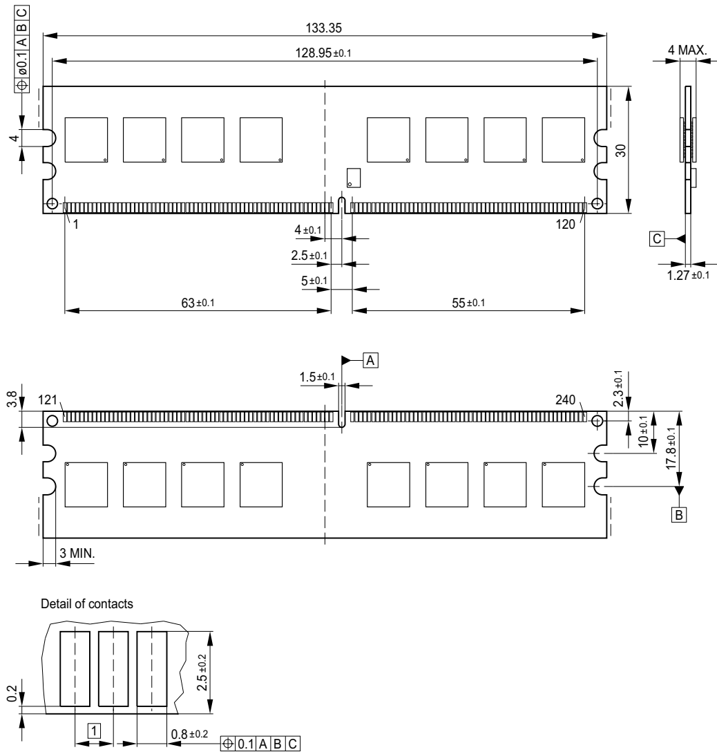
FIGURE 9 Package Outline Raw Card E L-DIM-240-9
