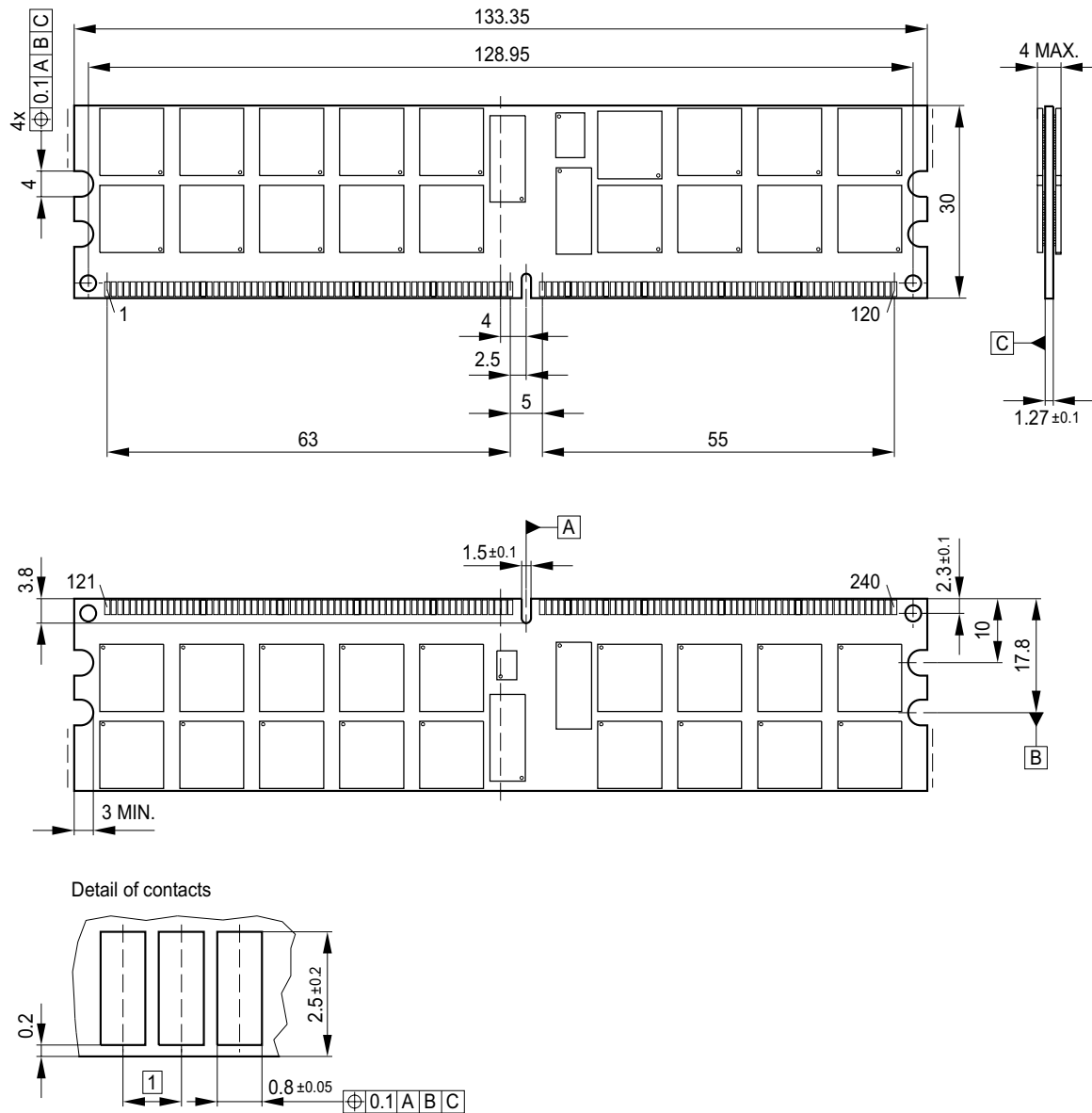
FIGURE 8 Package Outline Raw Card J L-DIM-240-20
