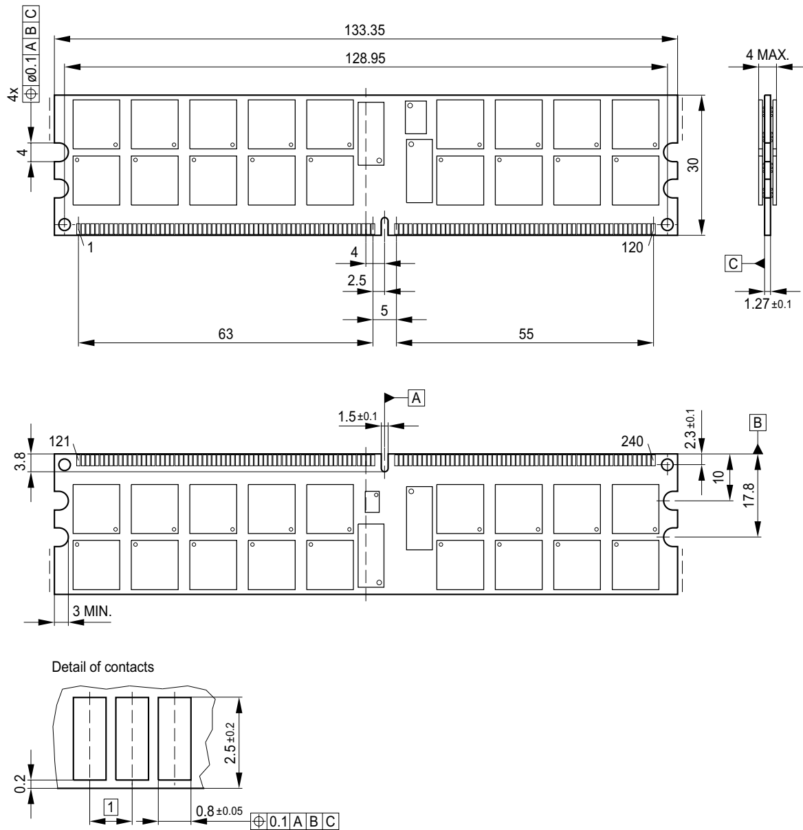
FIGURE 9 Package Outline Raw Card N L-DIM-240-44
