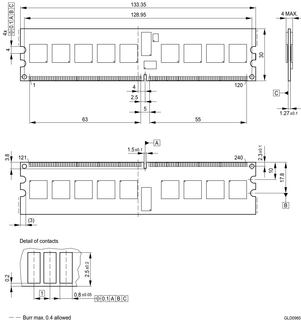
FIGURE 7 Package Outline Raw Card H L-DIM-240-13
