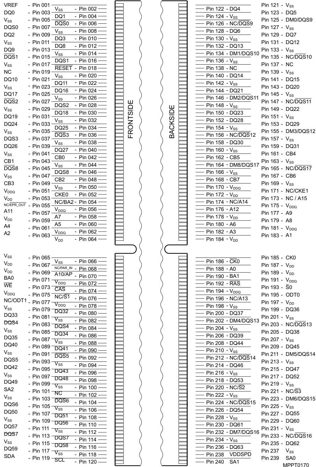
FIGURE 1 Pin Configuration for RDIMM (240 pins)
