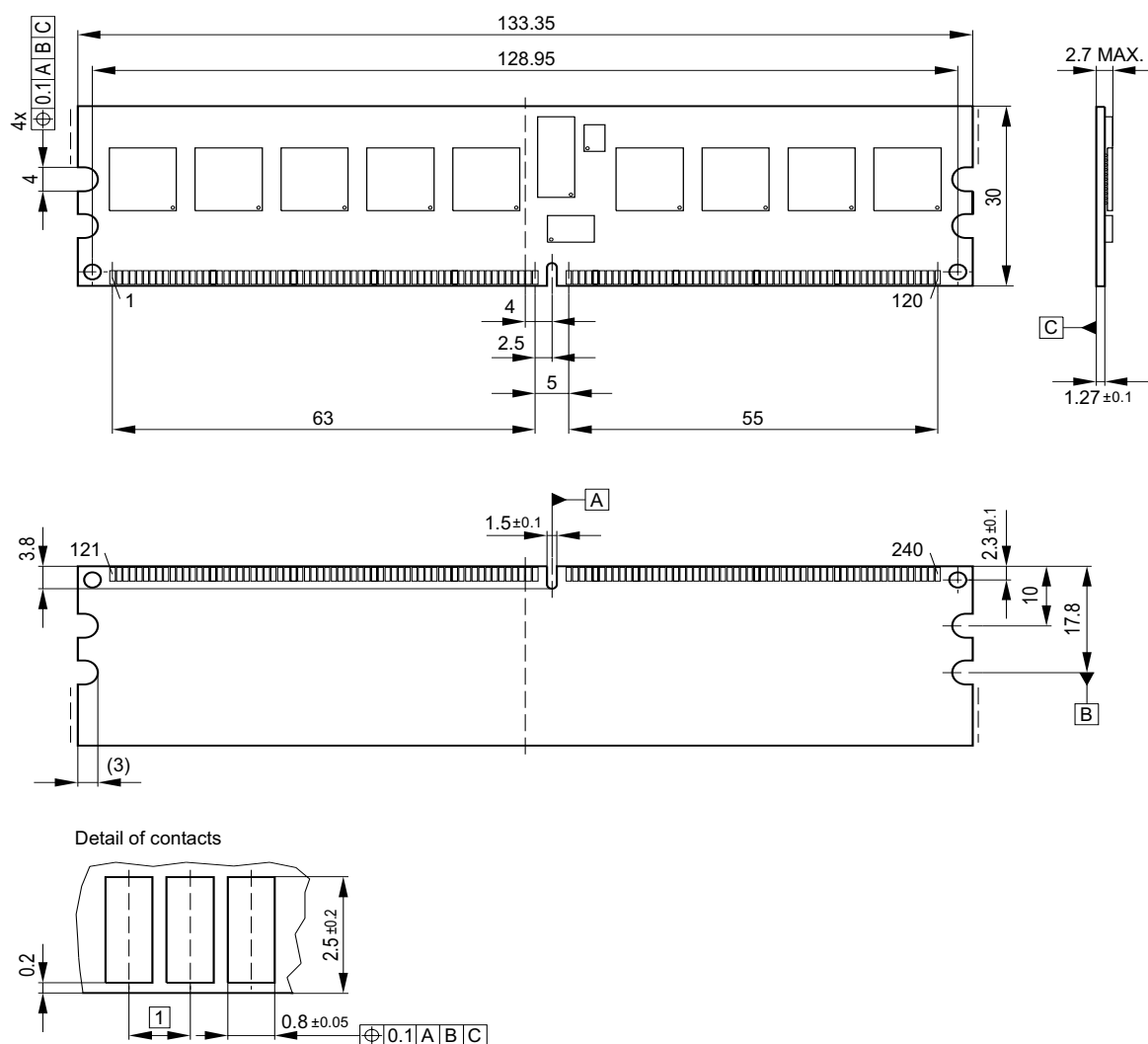
FIGURE 5 Package Outline Raw Card F L-DIM-240-11
