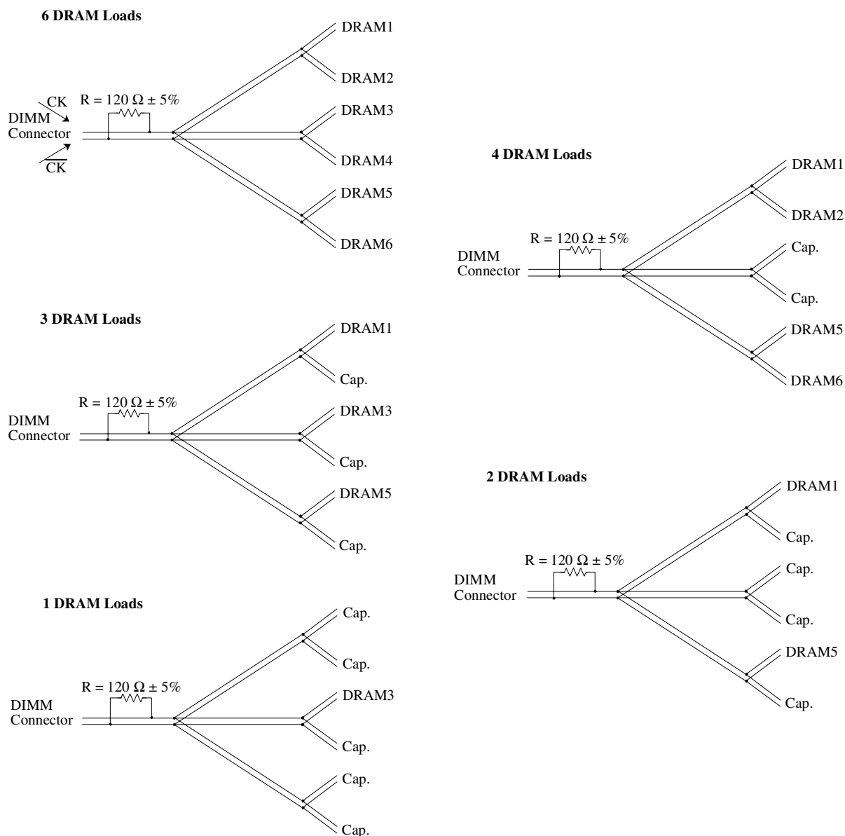
Figure 6 Clock Net Wiring
