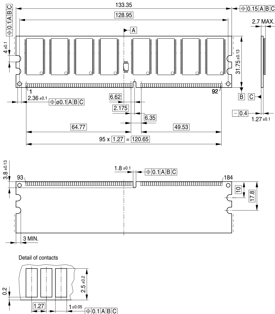
FIGURE 3 Raw Card A DDR UDIMM HYS64D64300HU-[5/6/7]-B (1 Rank Module)
