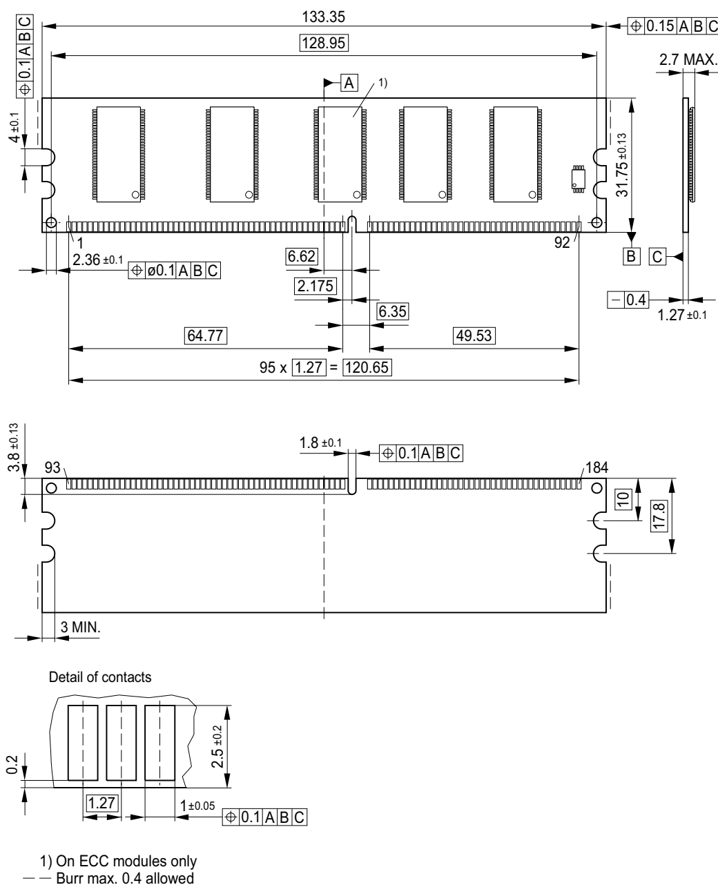
FIGURE 2 Raw Card C DDR UDIMM HYS64D32301HU-5-B (1 Rank Module)
