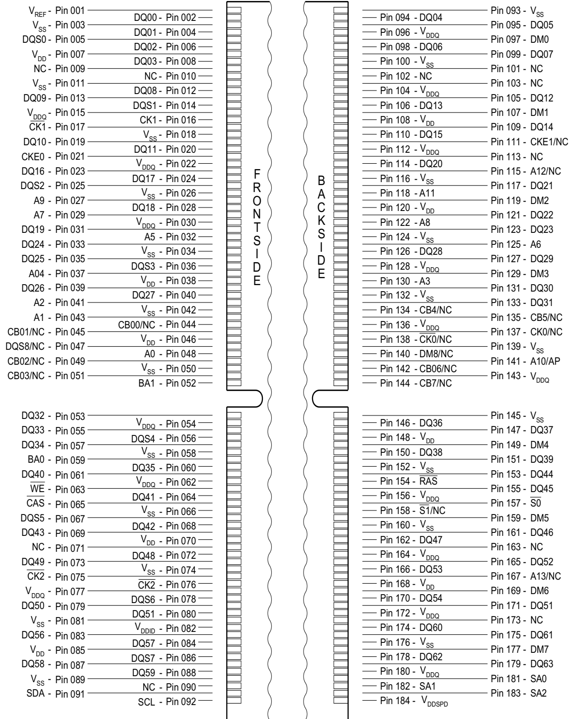
FIGURE 1 Pin Configuration 184-Pin, UDIMM
