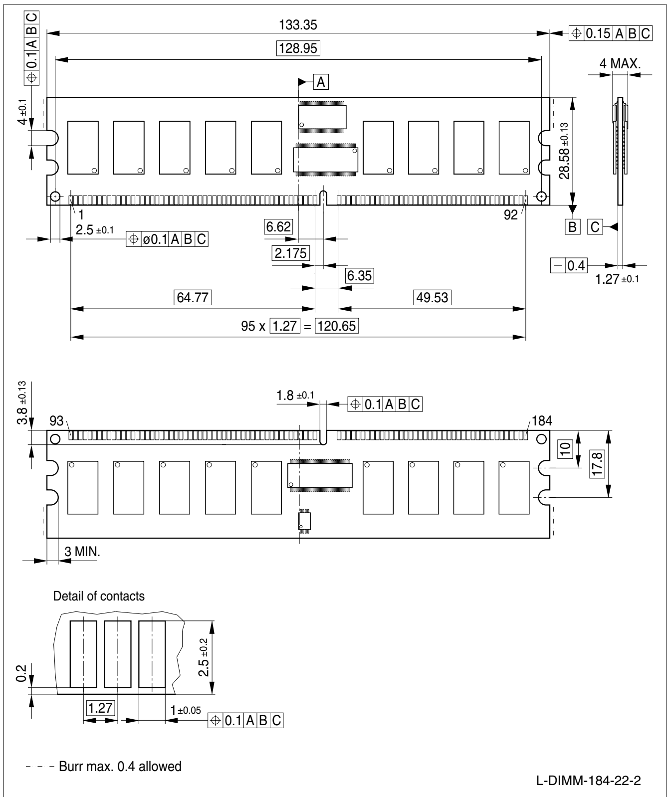
Figure 7 Package Outlines – Raw Card C HYS72D64300GBR-[5/6]-C (1 Rank × 4)
