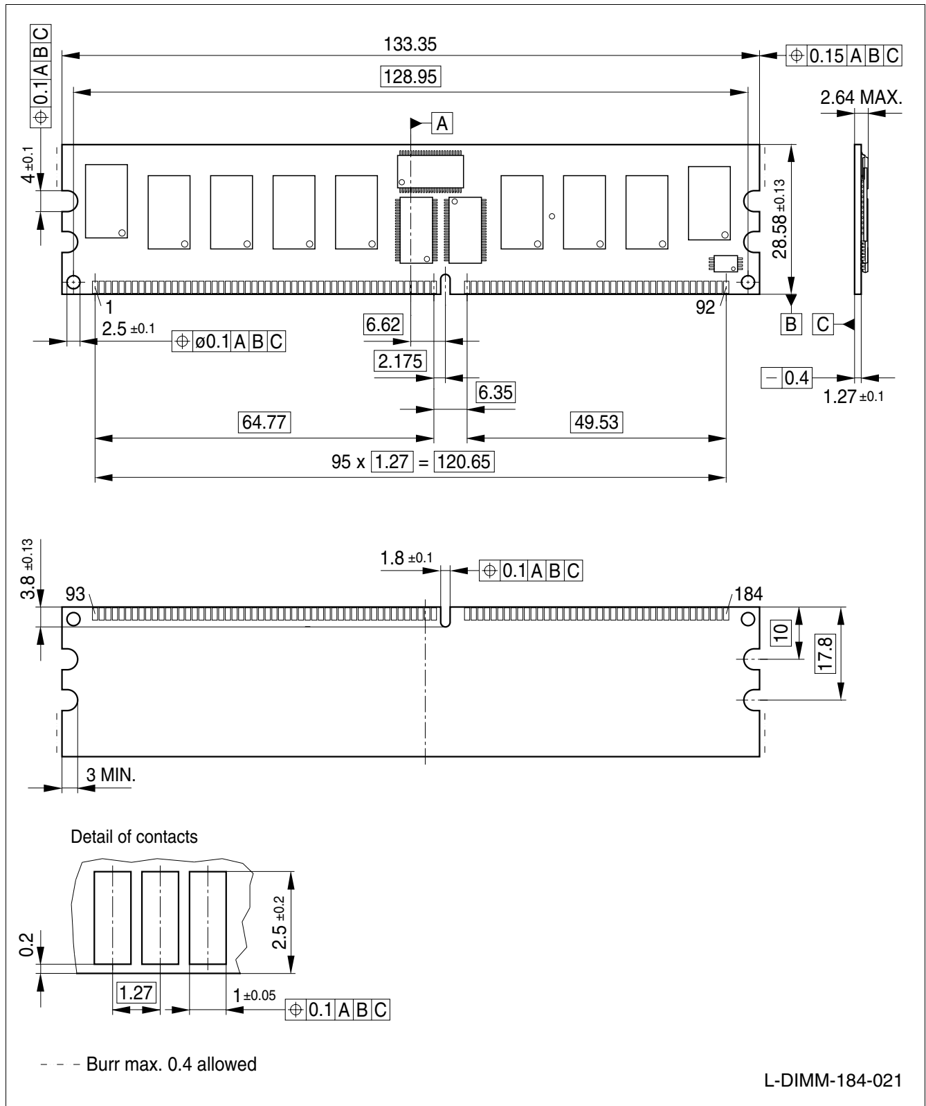
Figure 6 Package Outlines – Raw Card A HYS72D32300GBR-[5/6]-C (1 Rank x 8)
