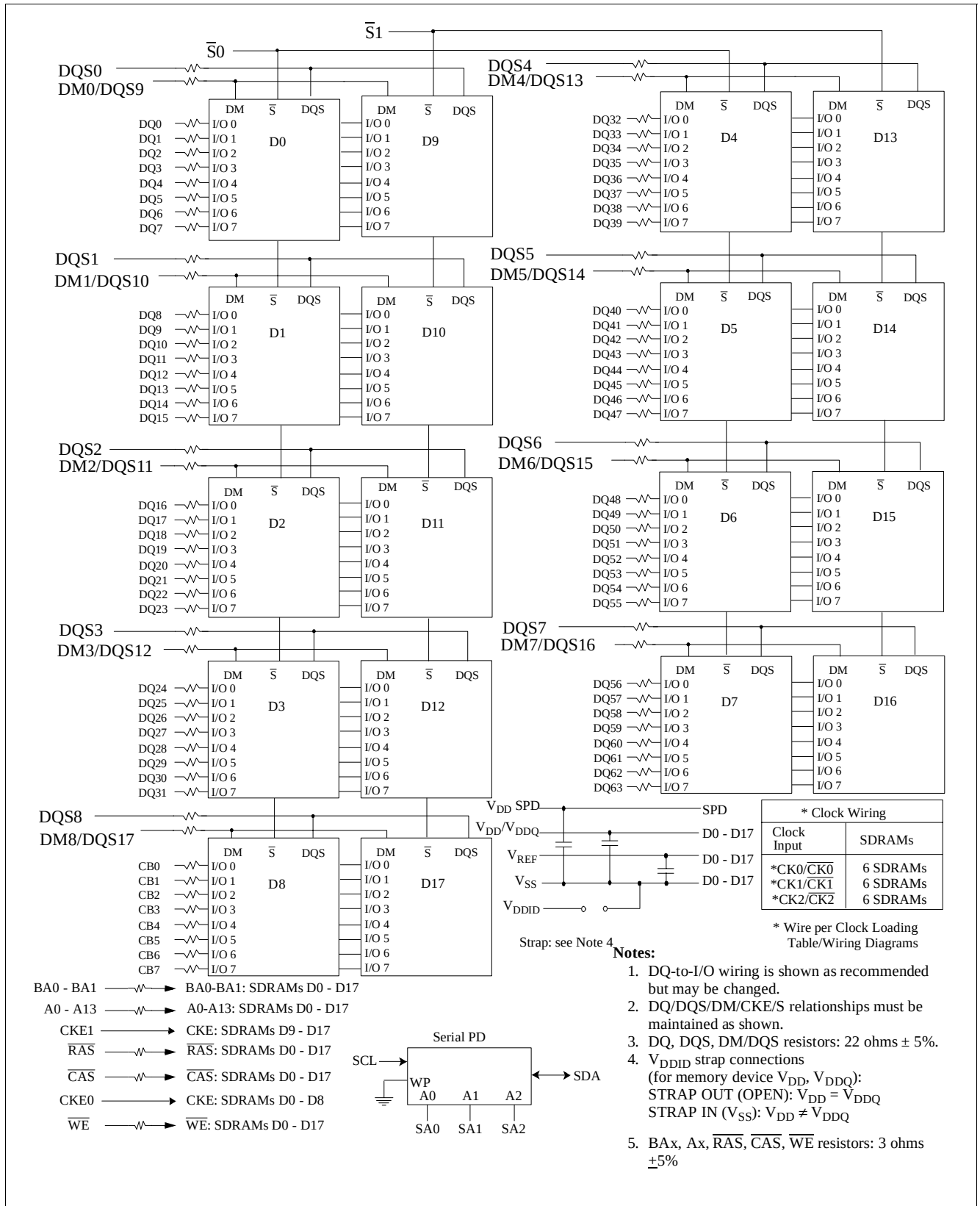
Figure 5 Block Diagram - Two Rank 64M \times 72 DDR-I SDRAM DIMM HYS72D64x20GU using \times 8 organized SDRAMs
