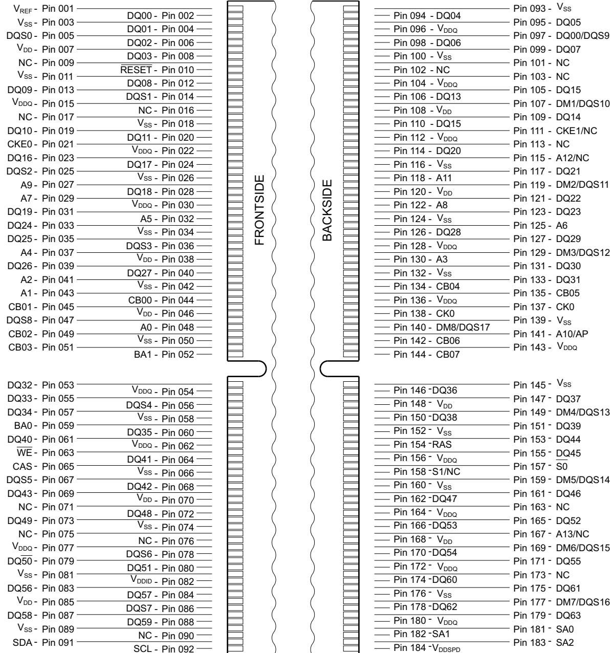
FIGURE 1 Pin Configuration 184 Pins, Reg
