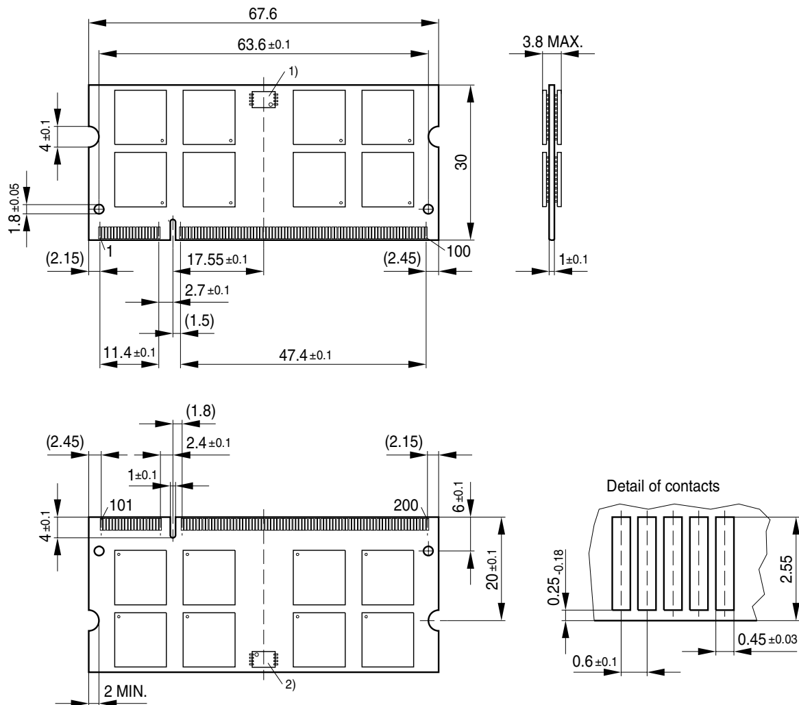
FIGURE 7 Package Outline L-DIM-200-36
