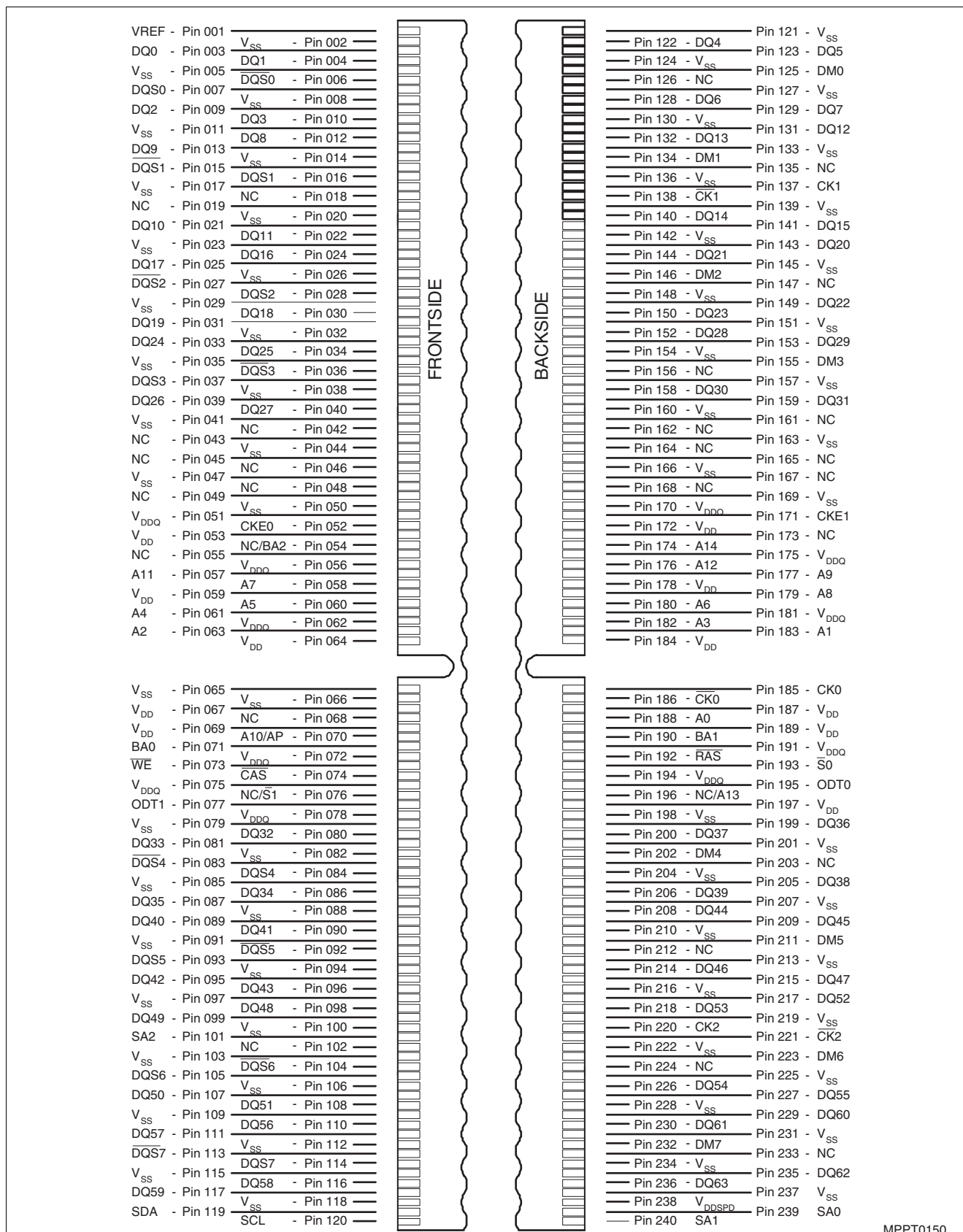
Figure 1 Pin Configuration UDIMM ×64 (240 Pin)
