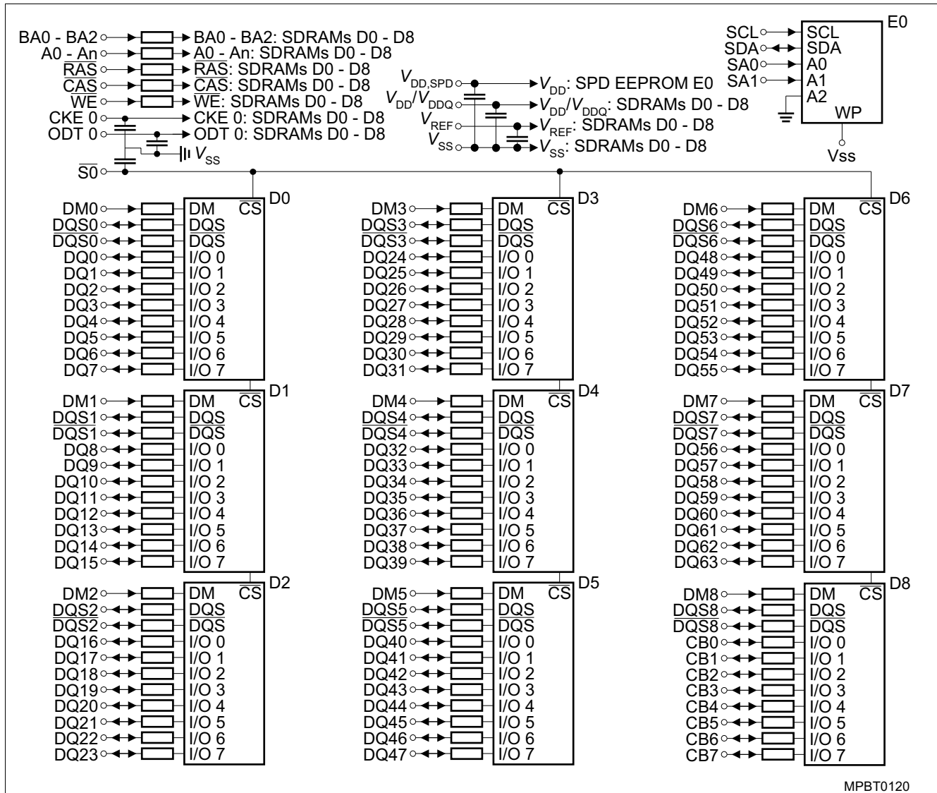
Figure 4 Block Diagram Raw Card A UDIMM (×72, 1 Rank, ×8)
