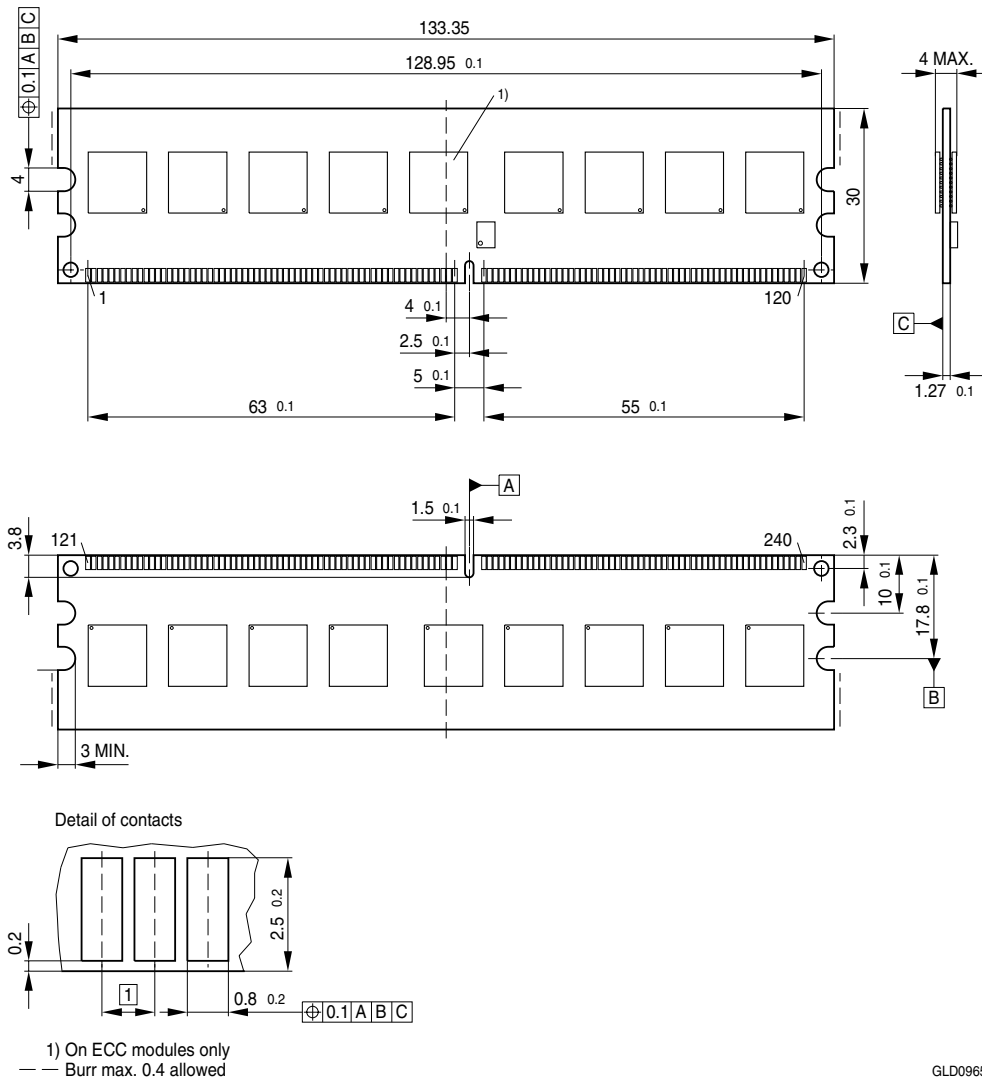
FIGURE 7 Package Outline Raw Card B L-DIM-240-2
