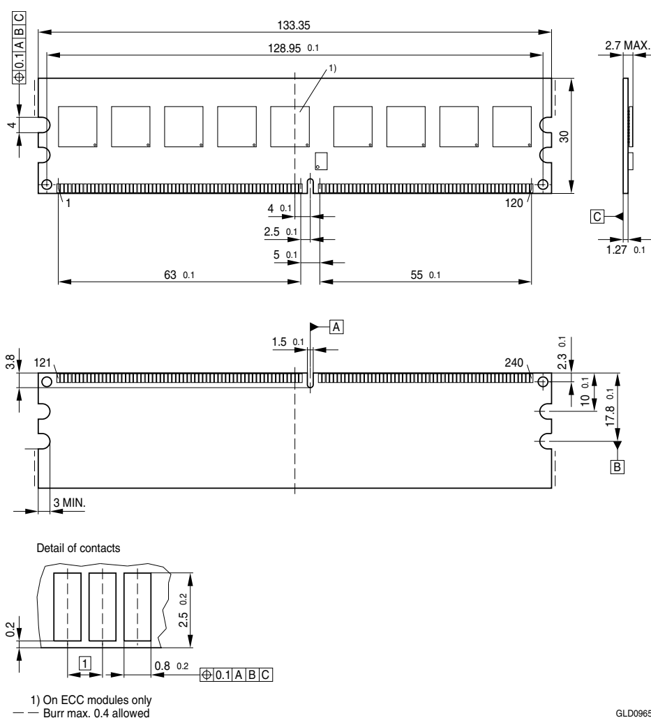
FIGURE 6 Package Outline Raw Card A L-DIM-240-1
