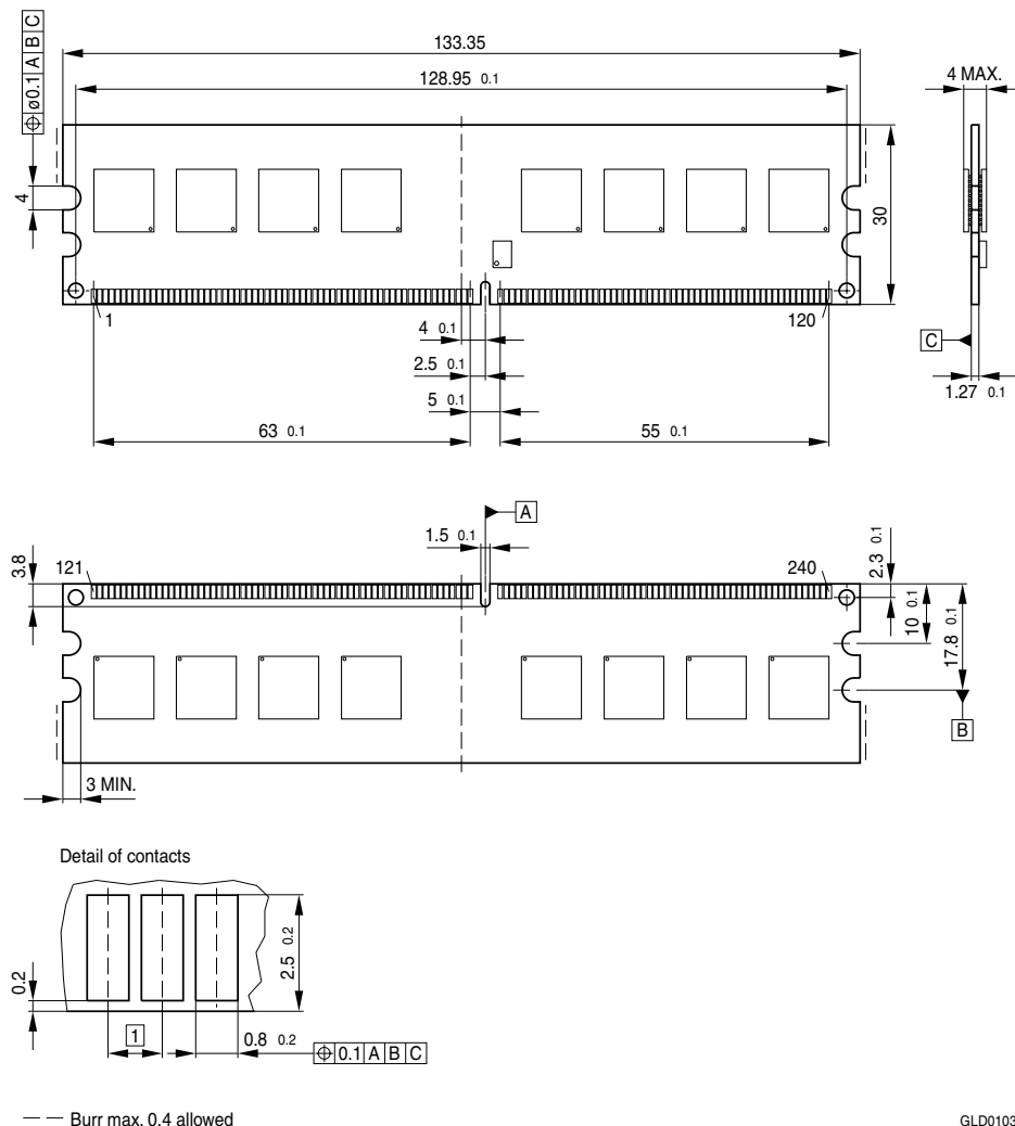
FIGURE 10 Package Outline L-DIM-240-9
