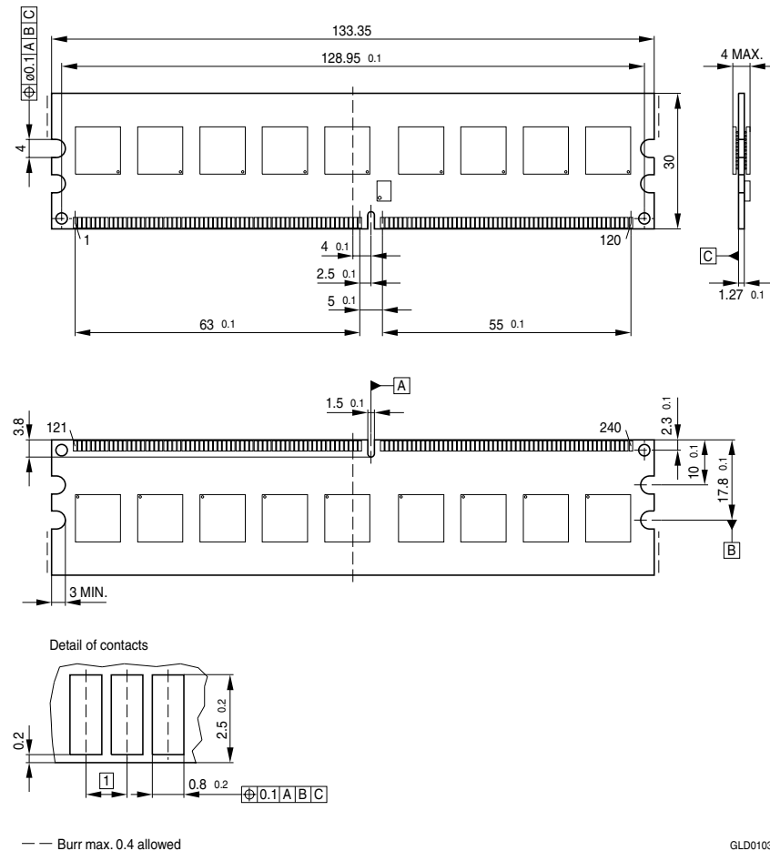
FIGURE 12 Package Outline Raw Card G L-DIM-240-7
