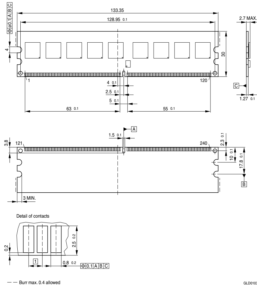
FIGURE 11 Package Outline Raw Card F L-DIM-240-6
