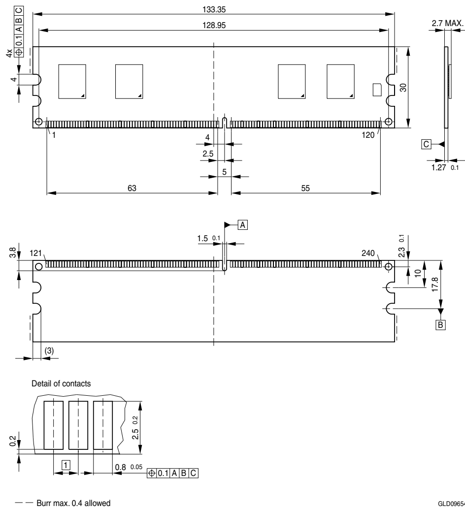
FIGURE 8 Package Outline Raw Card C L-DIM-240-3
