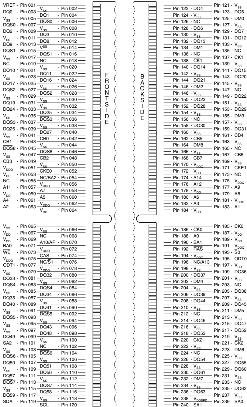
FIGURE 2 Pin Configuration UDIMM ×72 (240 Pin)
