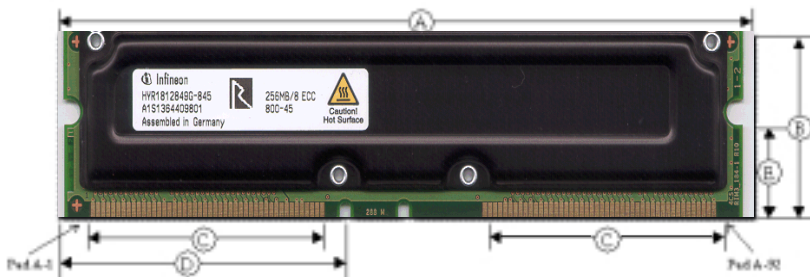
Fig.2 : RIMM Module PCB Physical Description
