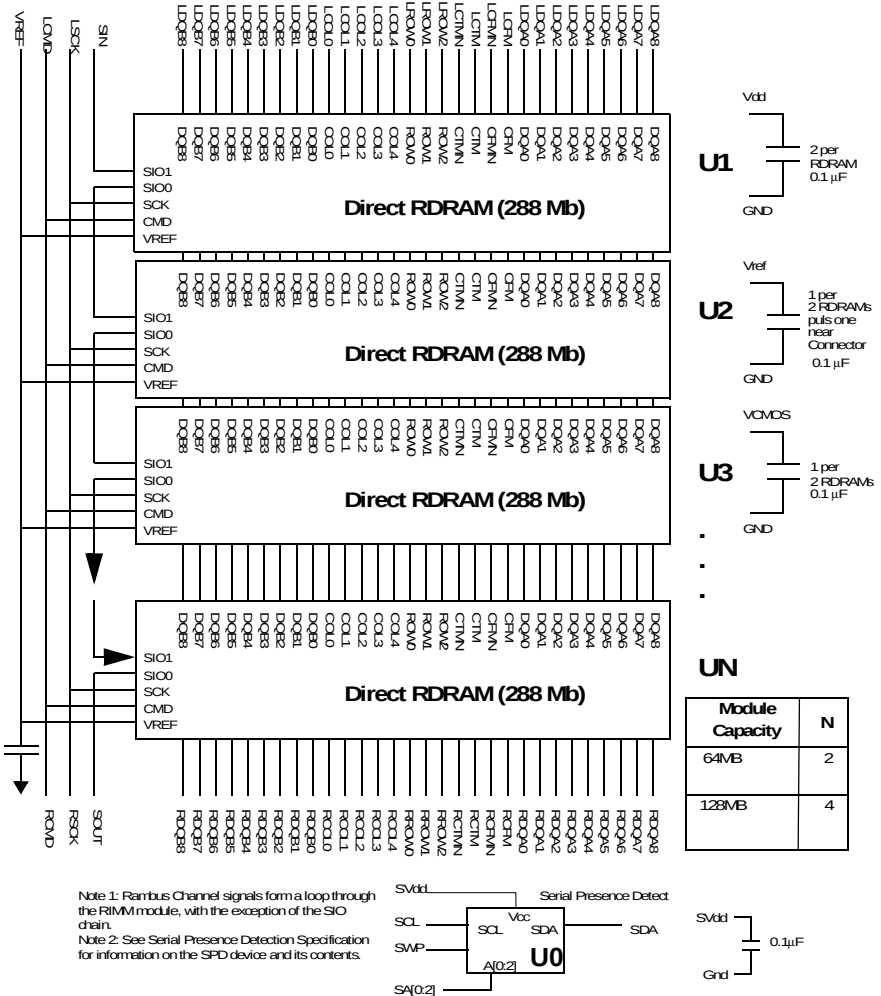
RIMM Module Functional Diagram
